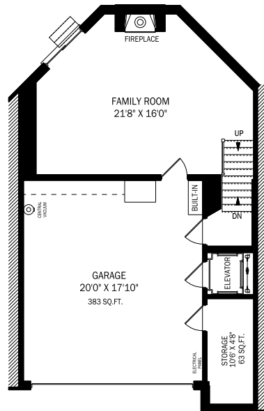
GROUND LEVEL - 417 SQUARE FEET
