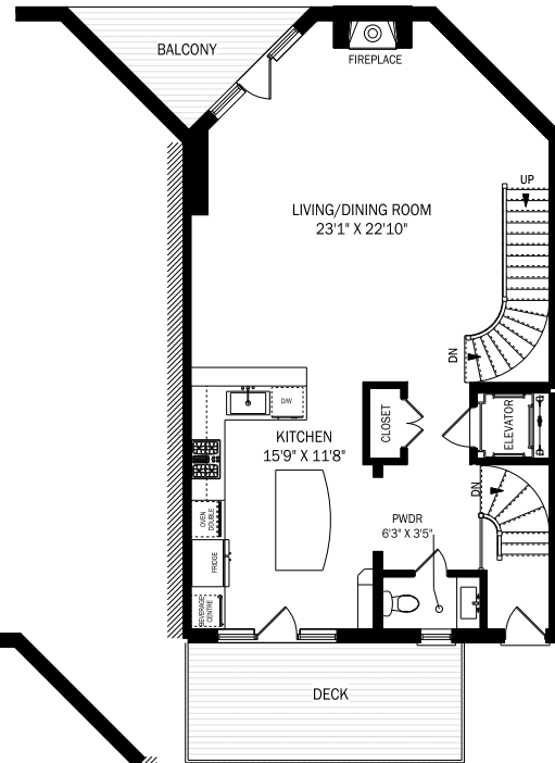
MAIN LEVEL - 905 SQUARE FEET
