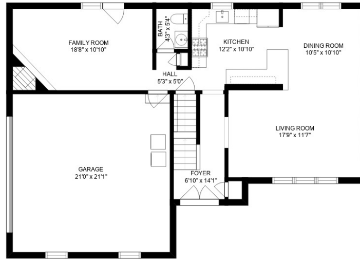
MAIN FLOOR
