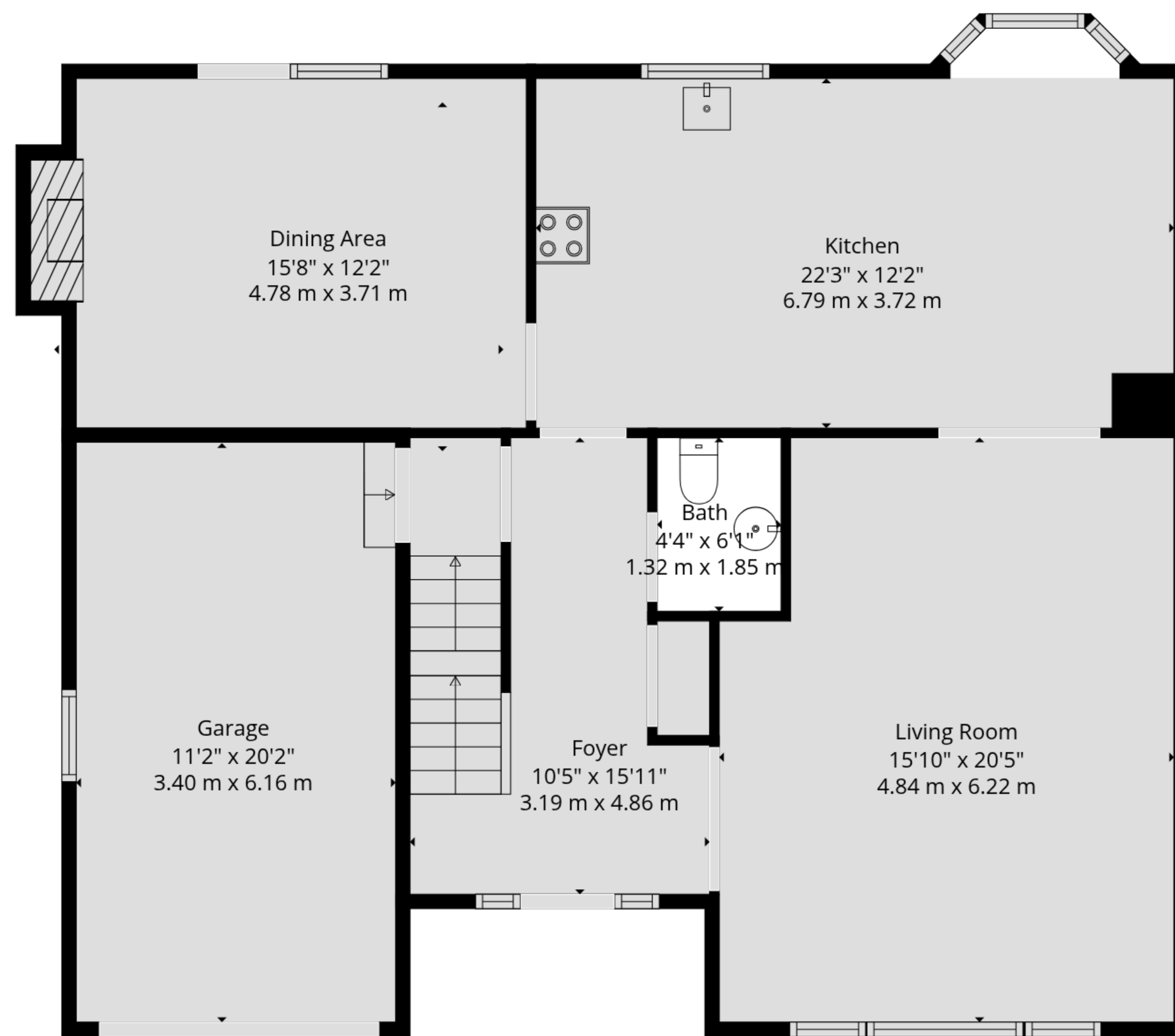
2nd Floor
