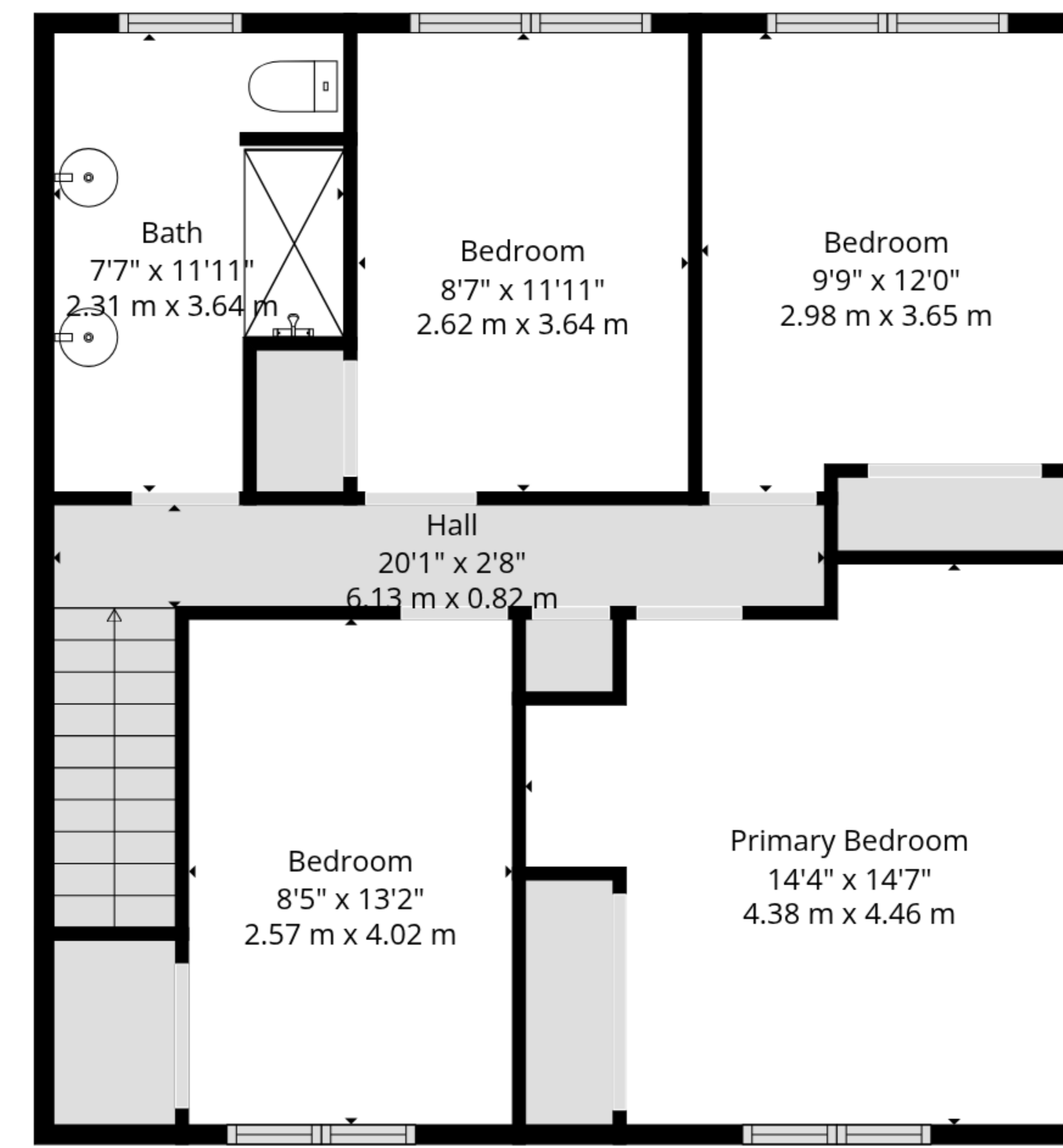
3rd Floor
