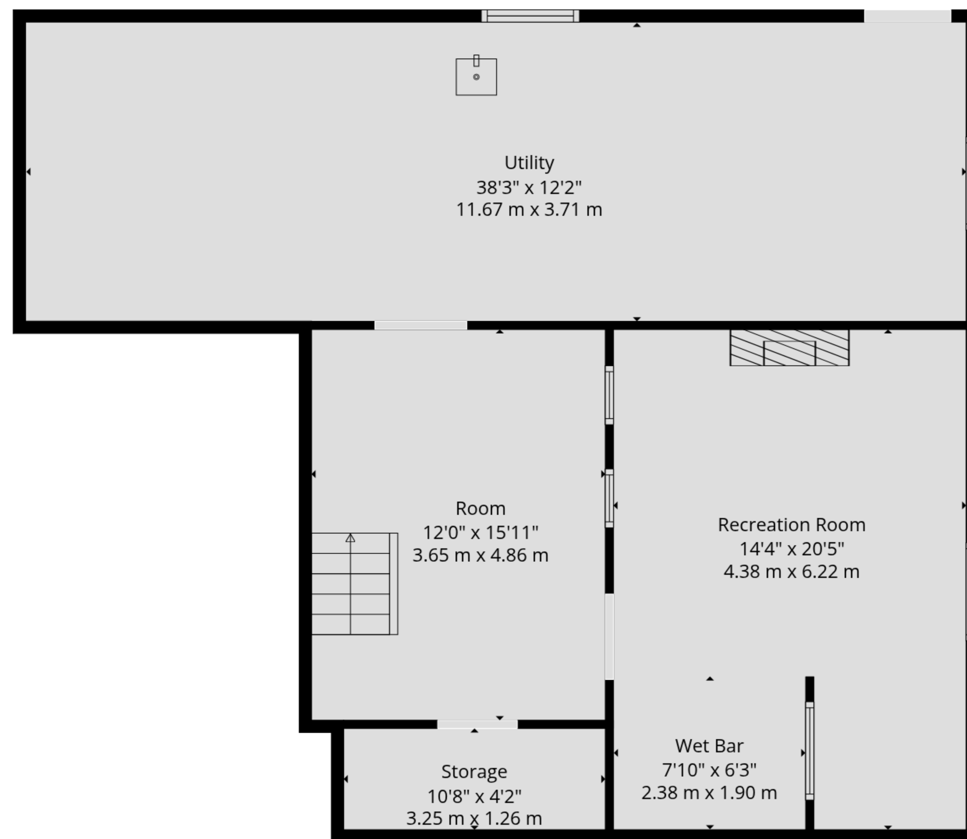
1st Floor
