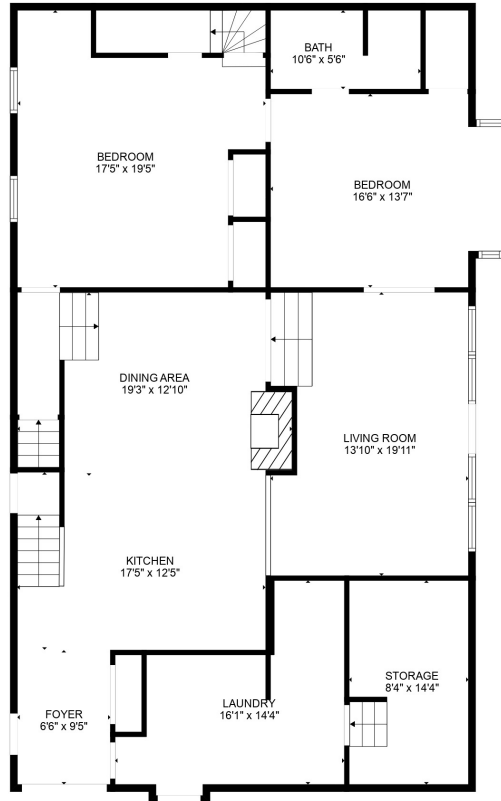
FLOOR 2
