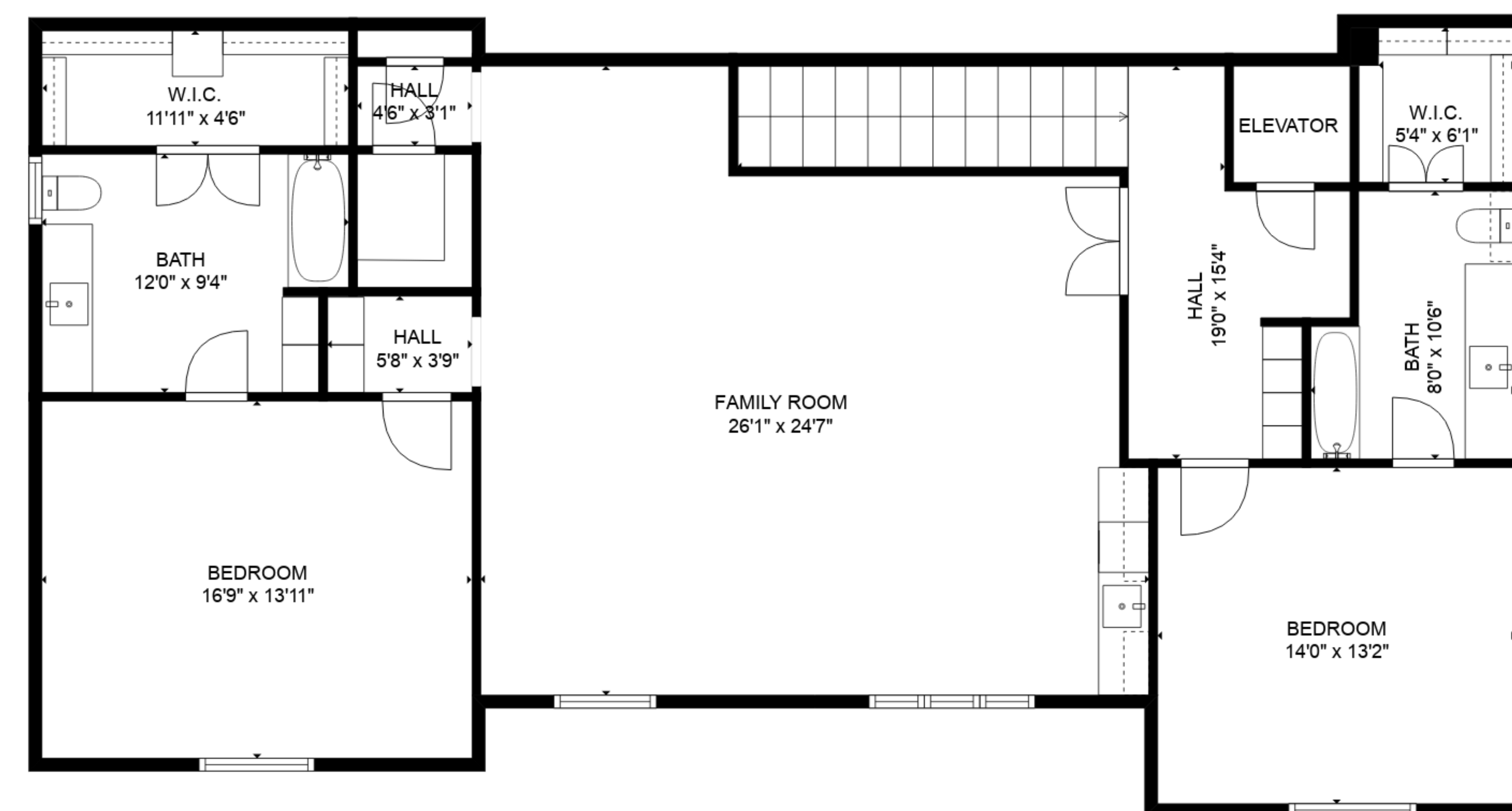
FLOOR 2
