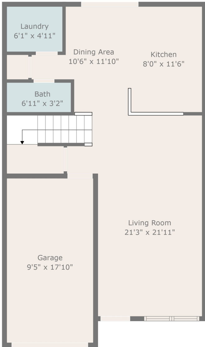
Floor 1
