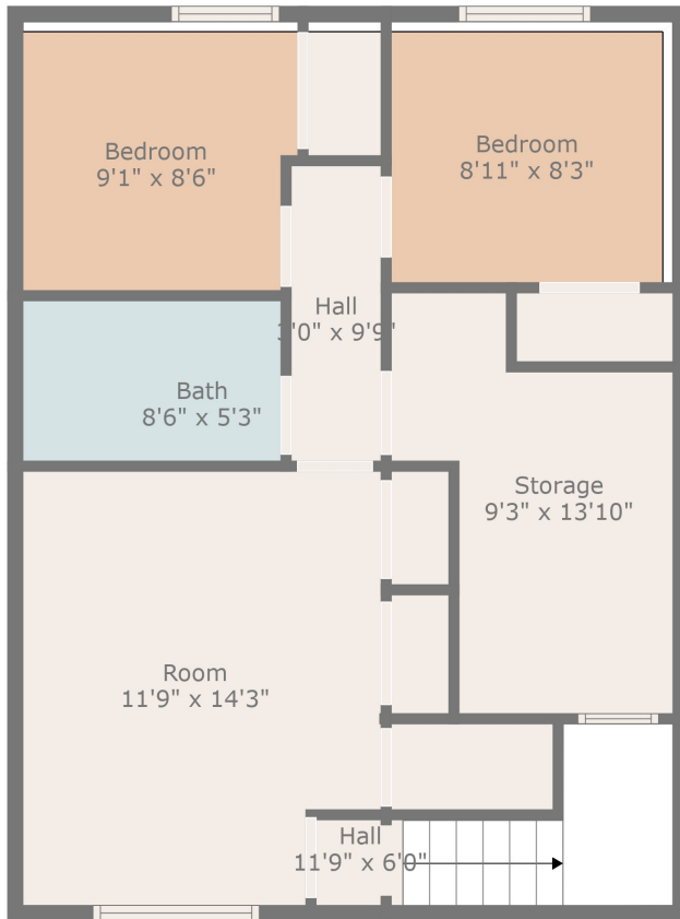
Floor 1
