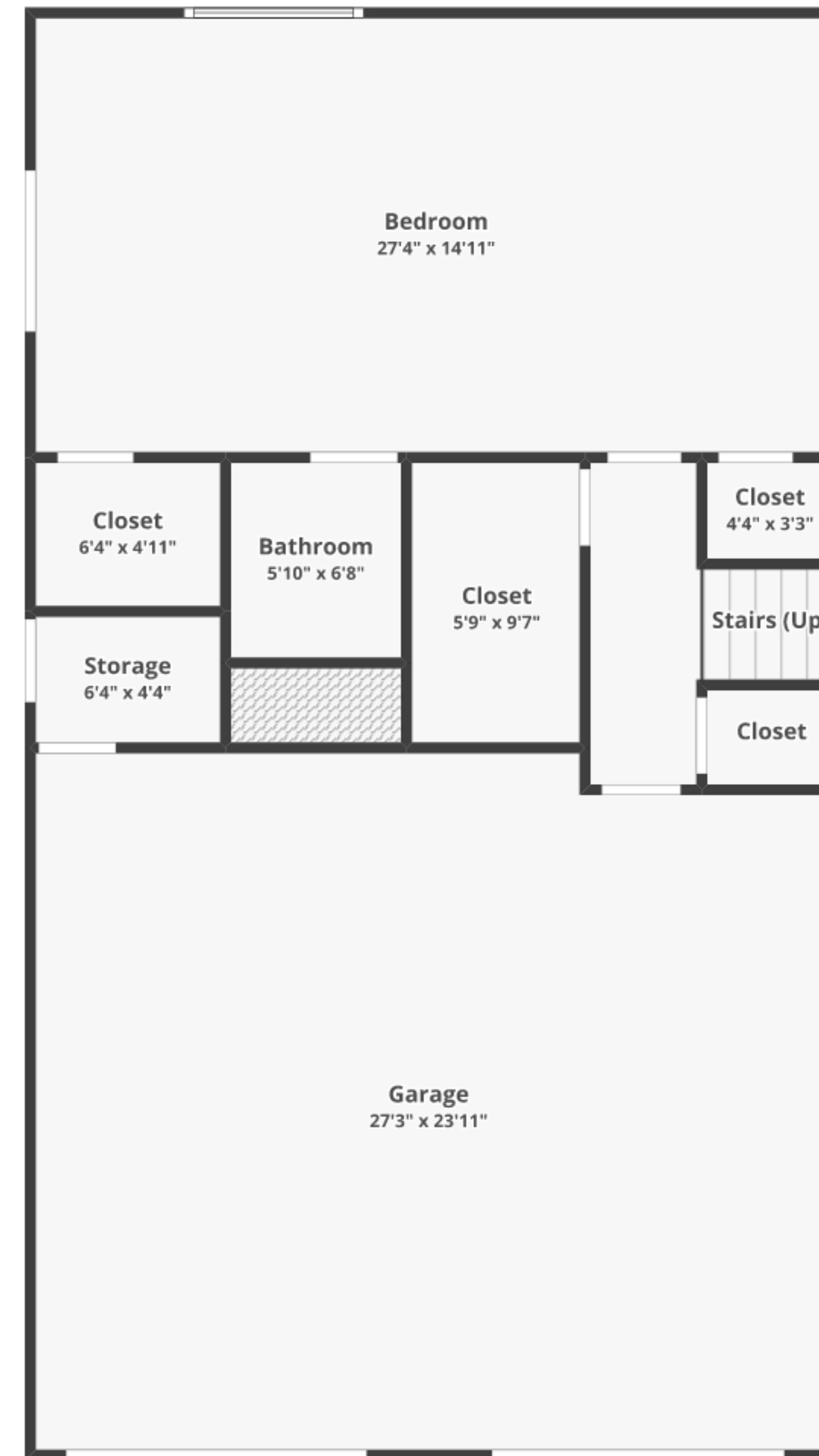
FLOOR 1
