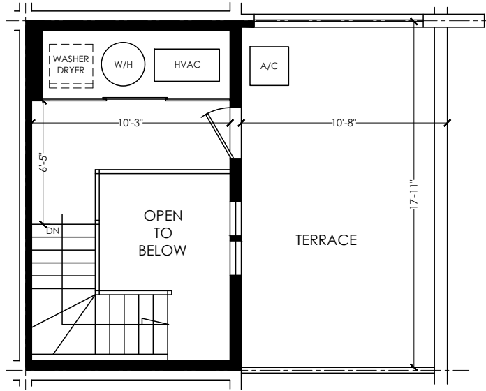
THIRD FLOOR FLOOR AREA 99 SQUARE FEET
