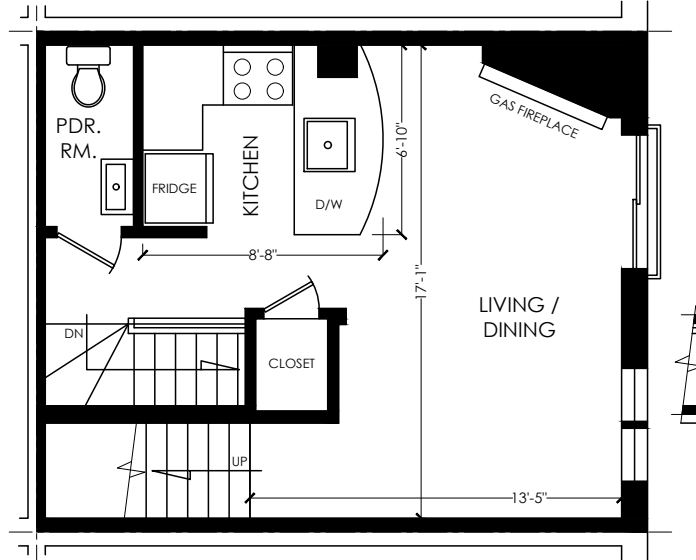
MAIN FLOOR FLOOR AREA AND ENTRY 436 SQUARE FEET
