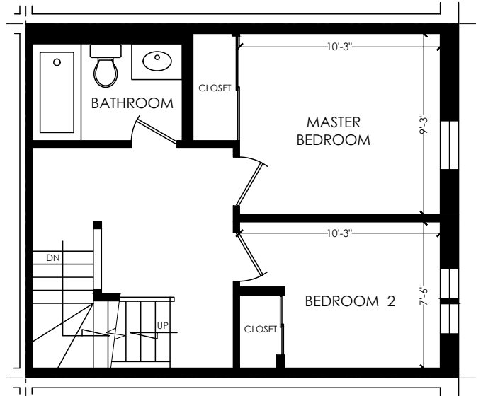
SECOND FLOOR FLOOR AREA 400 SQUARE FEET
