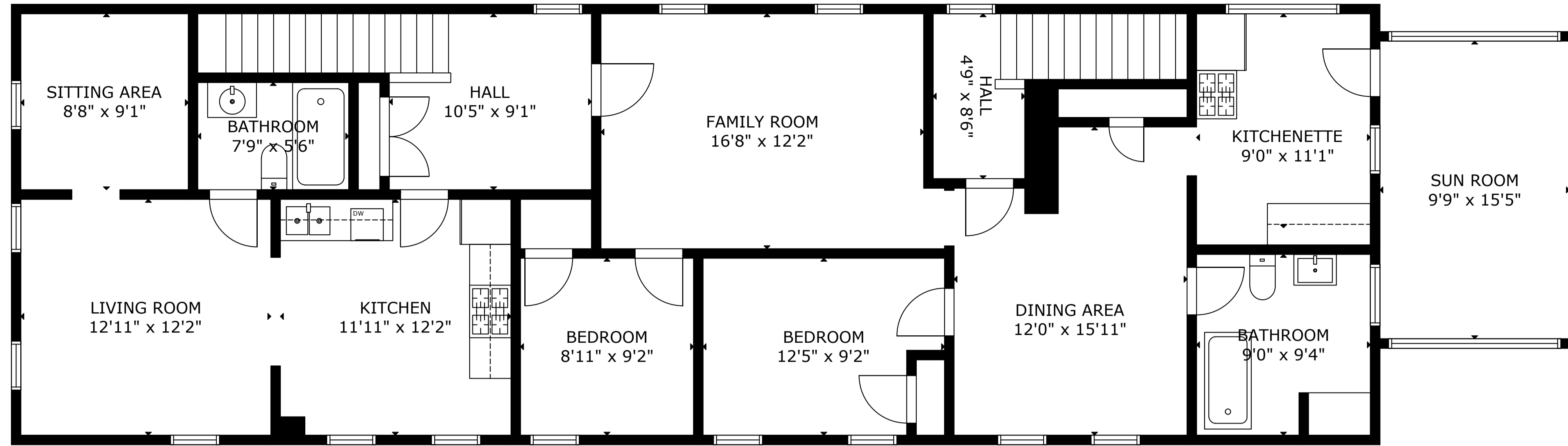
SECOND FLOOR
