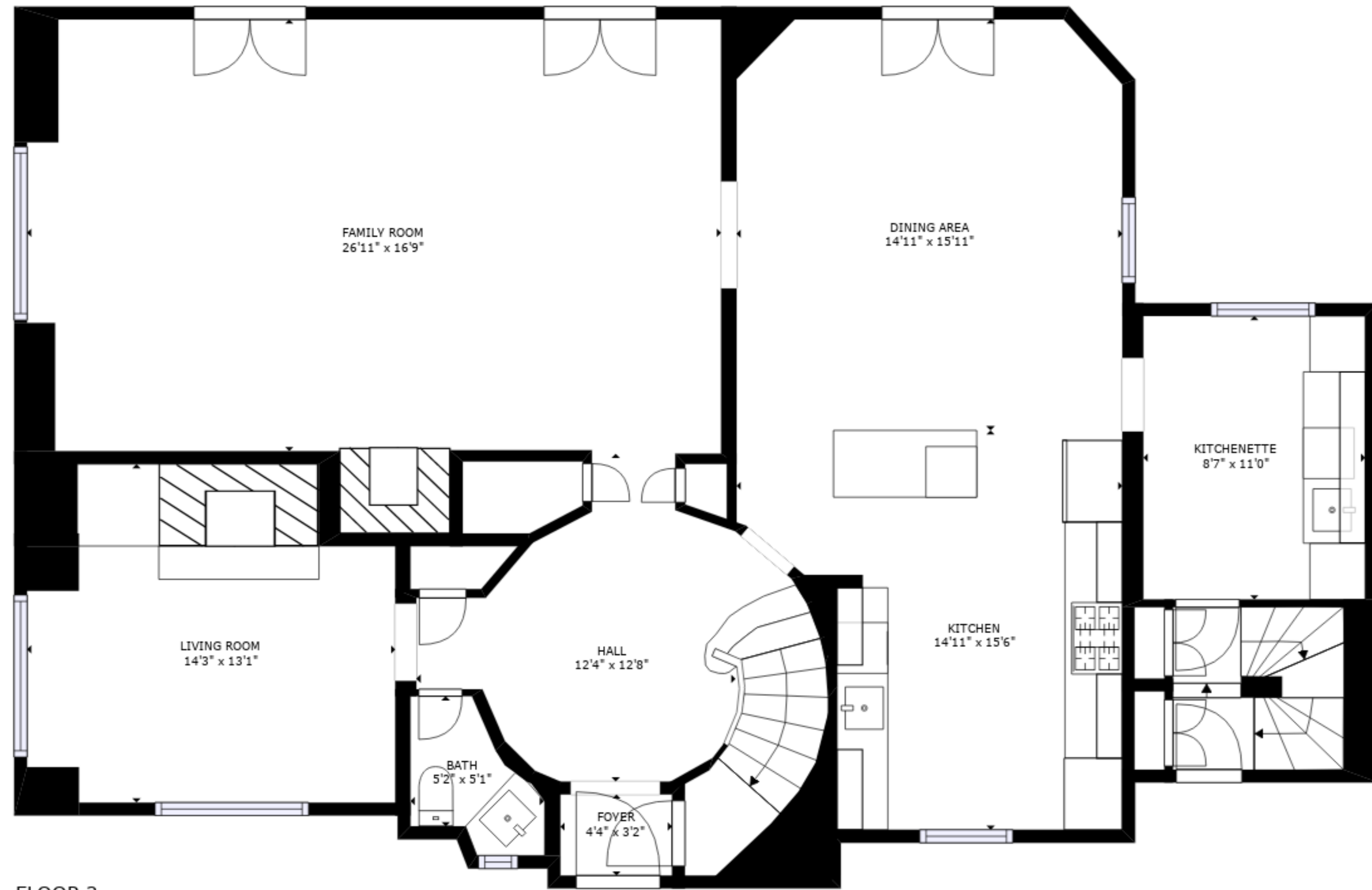
FLOOR 2
