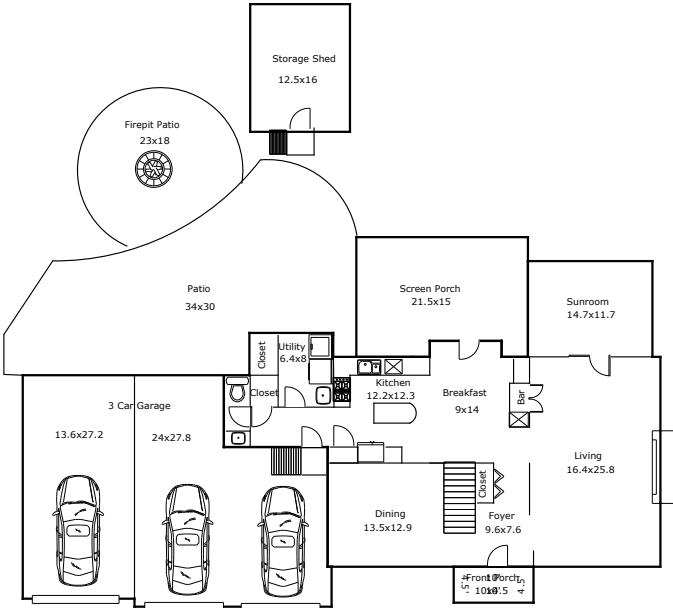
1st Floor
