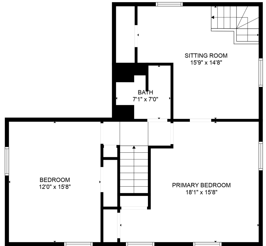
FLOOR 2
