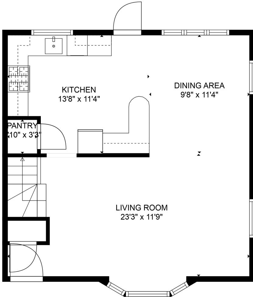
FLOOR 1
