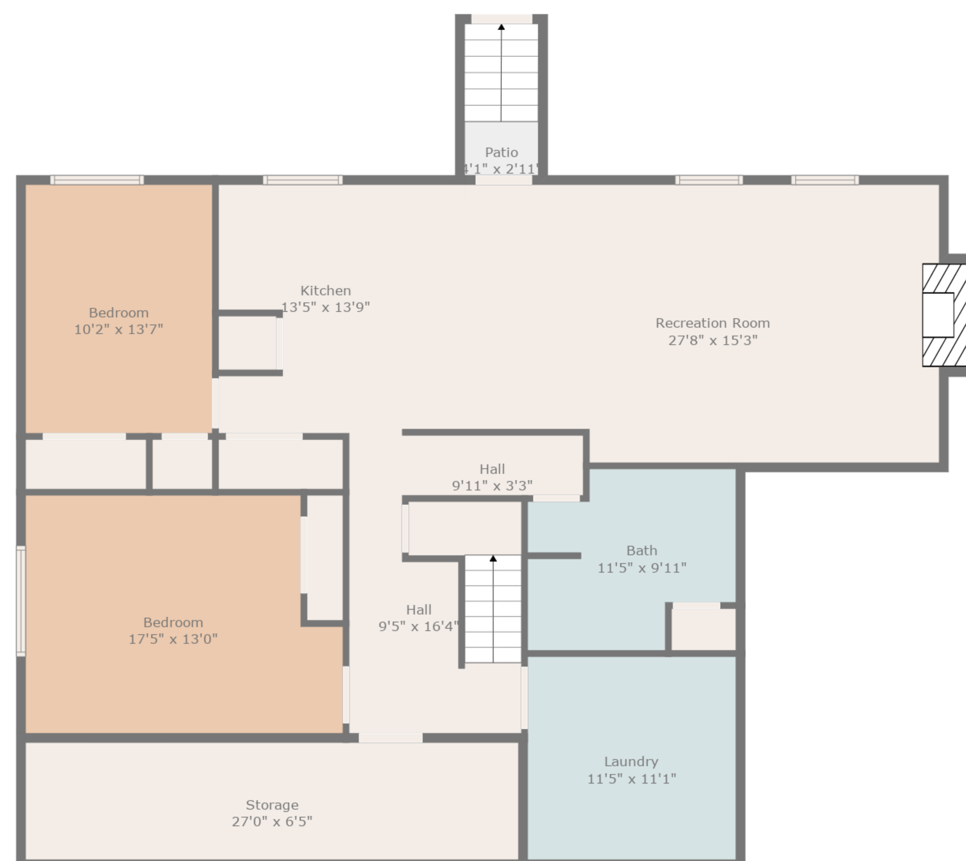
Floor 1
