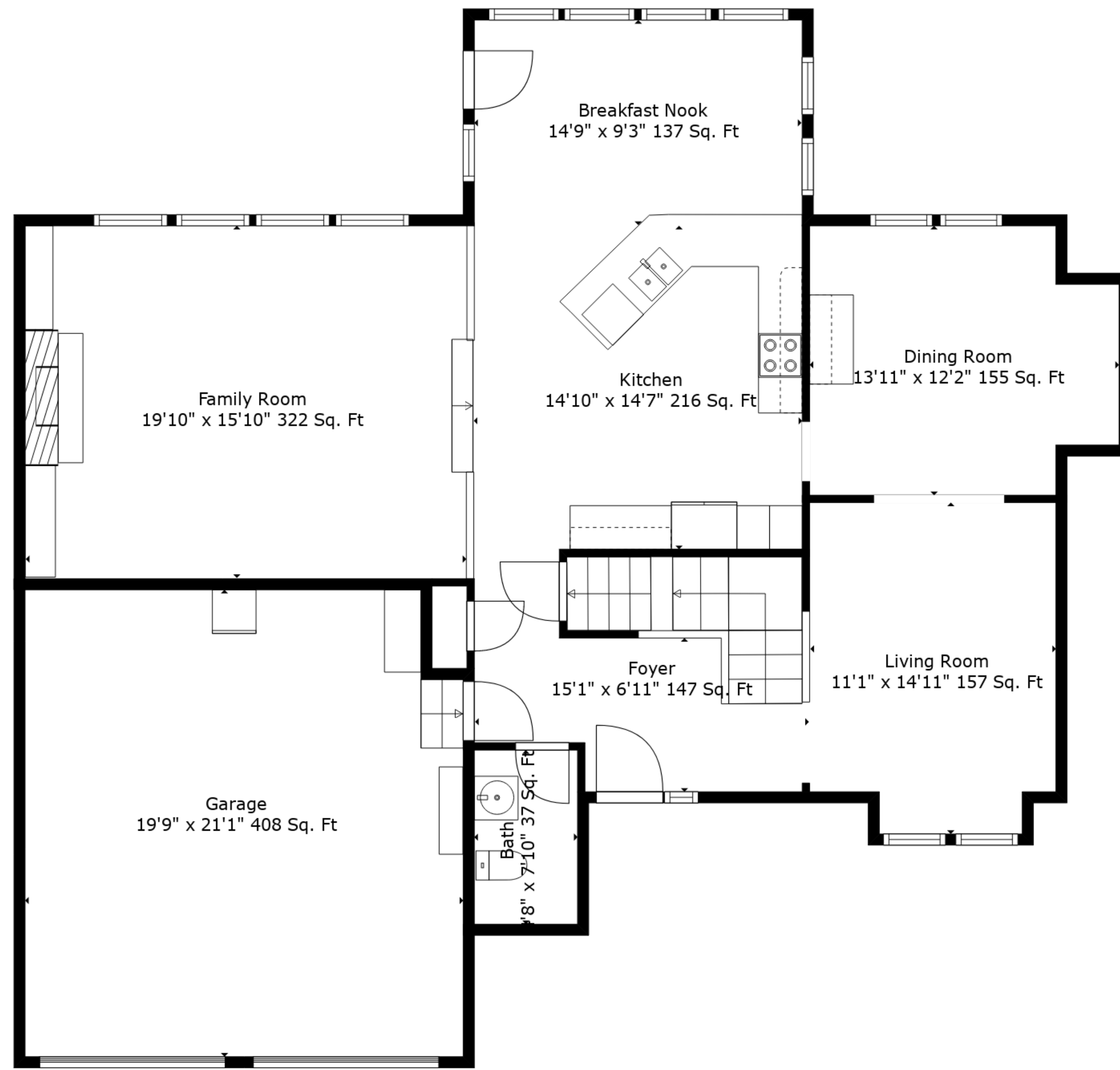
Floor 2
