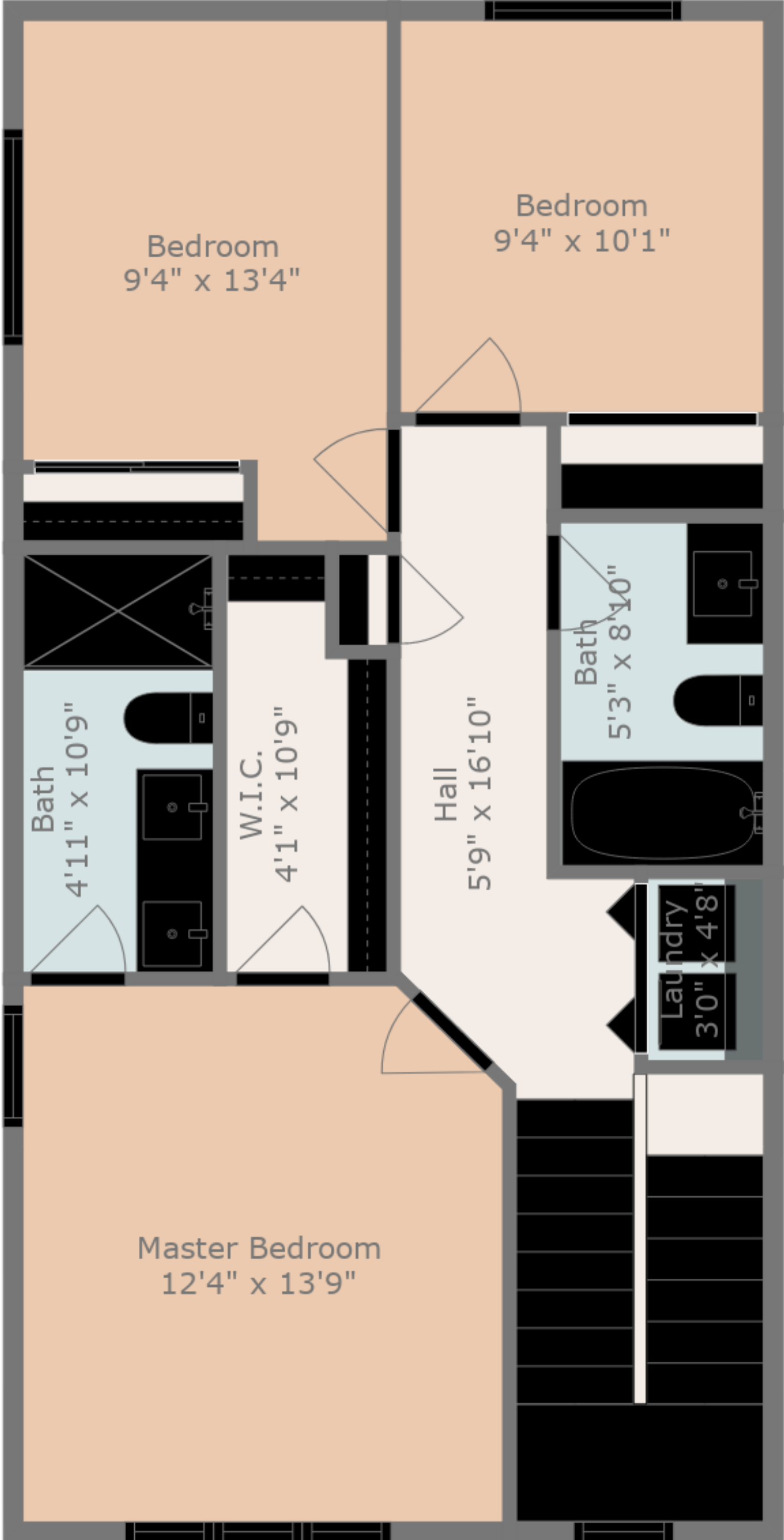
Floor 3
