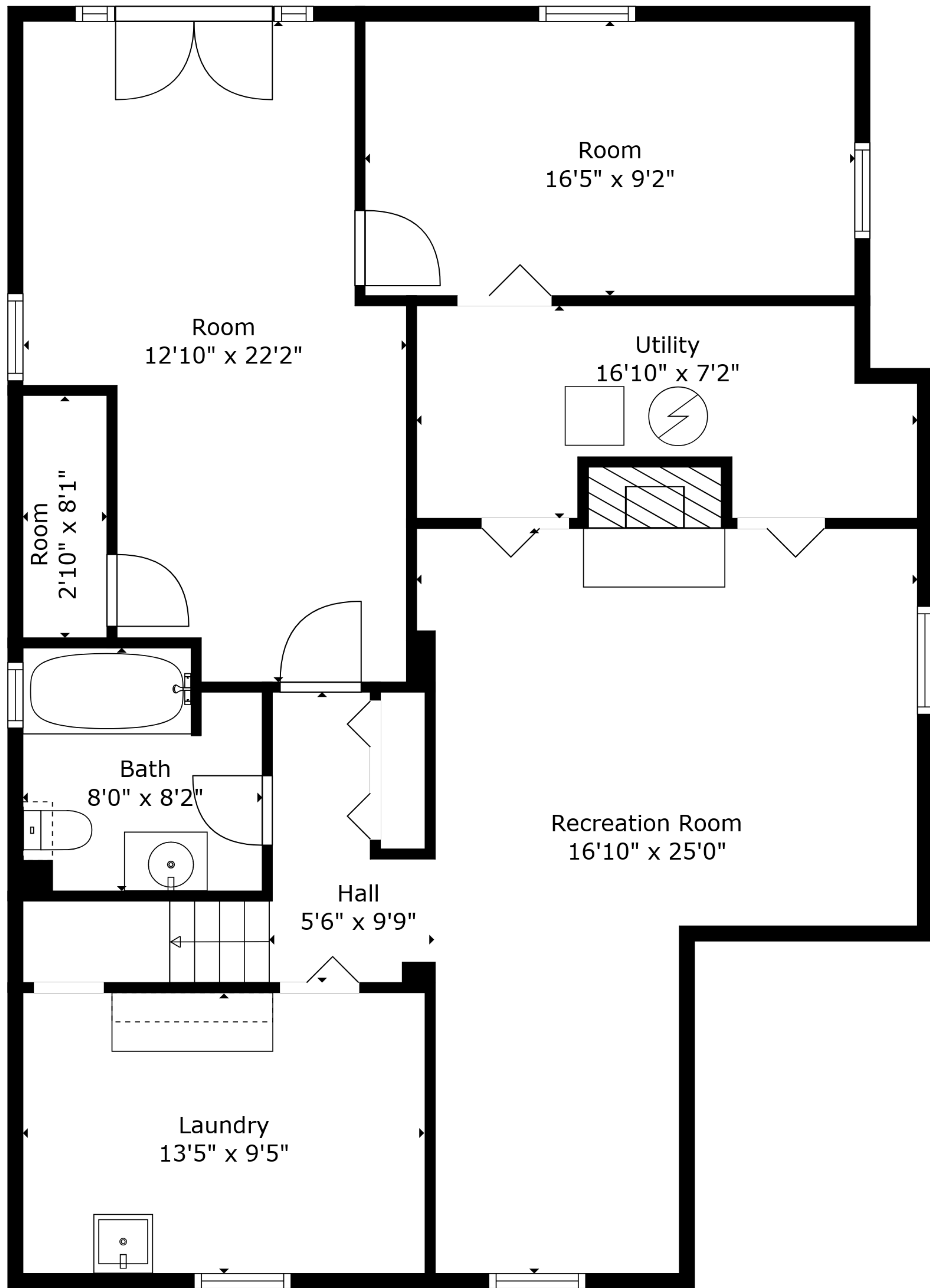
Floor 1
