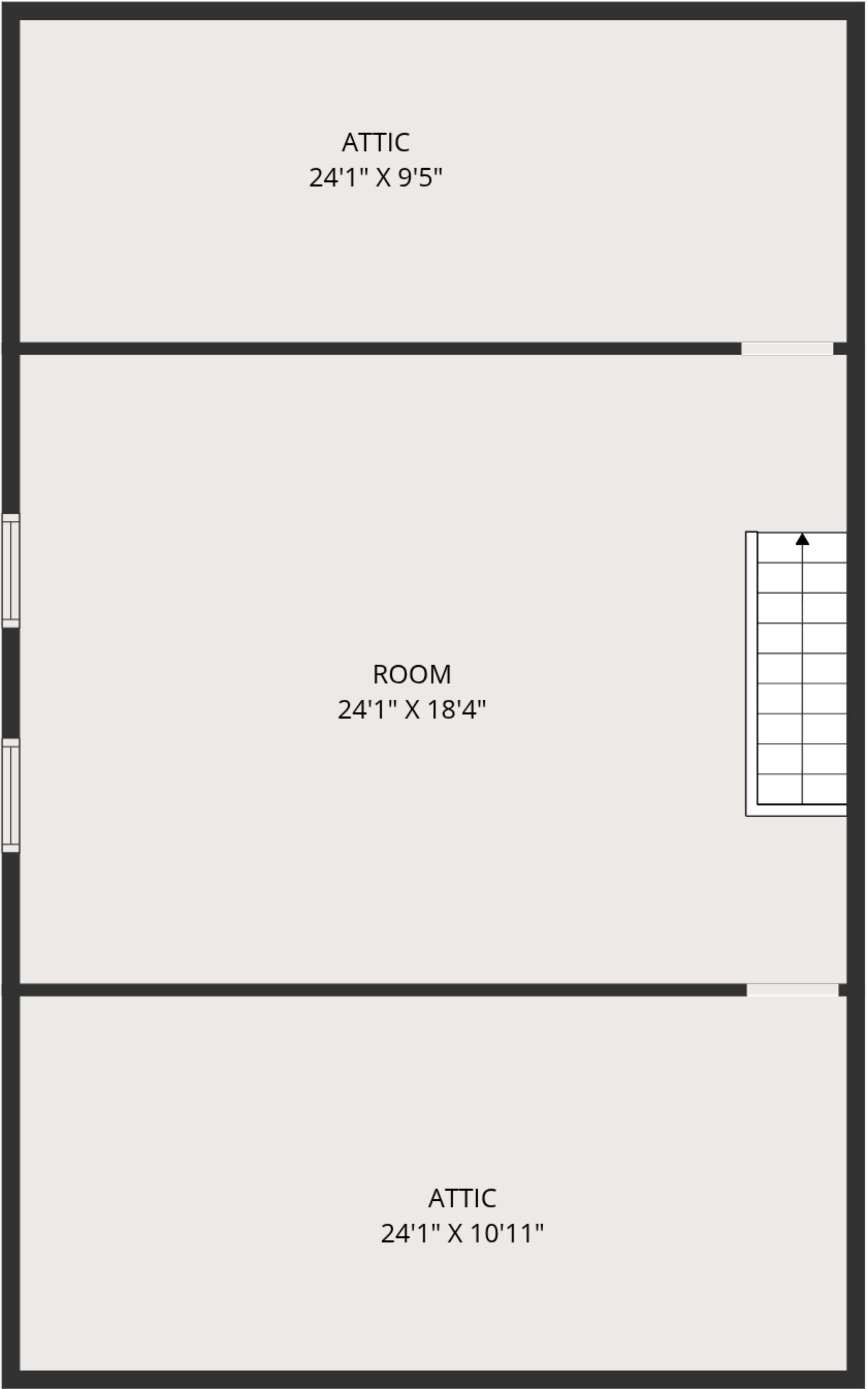
3RD FLOOR
