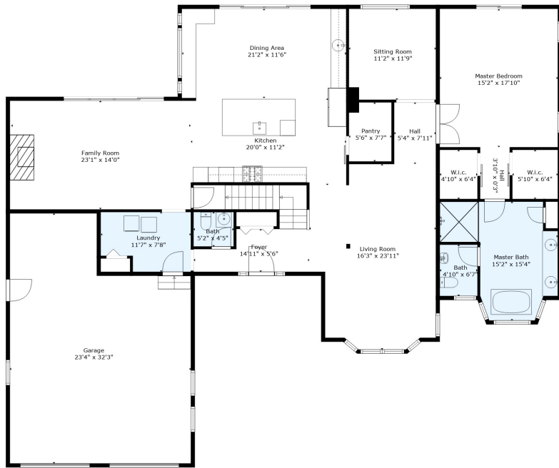
Floor 2
