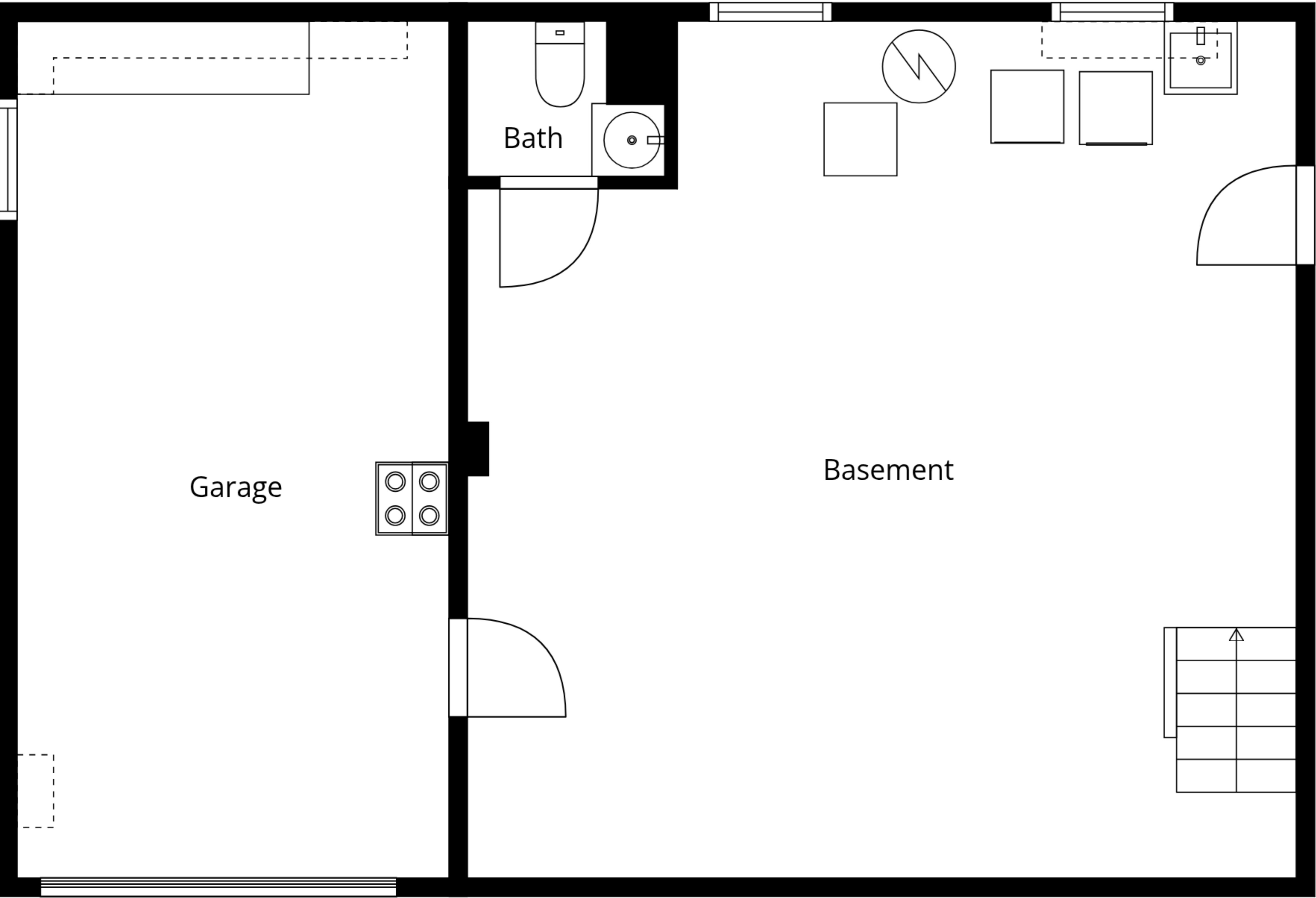
1st Floor
