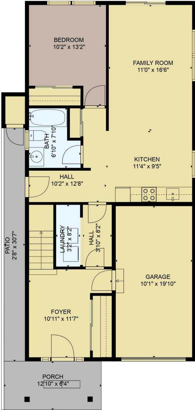
FLOOR 1
