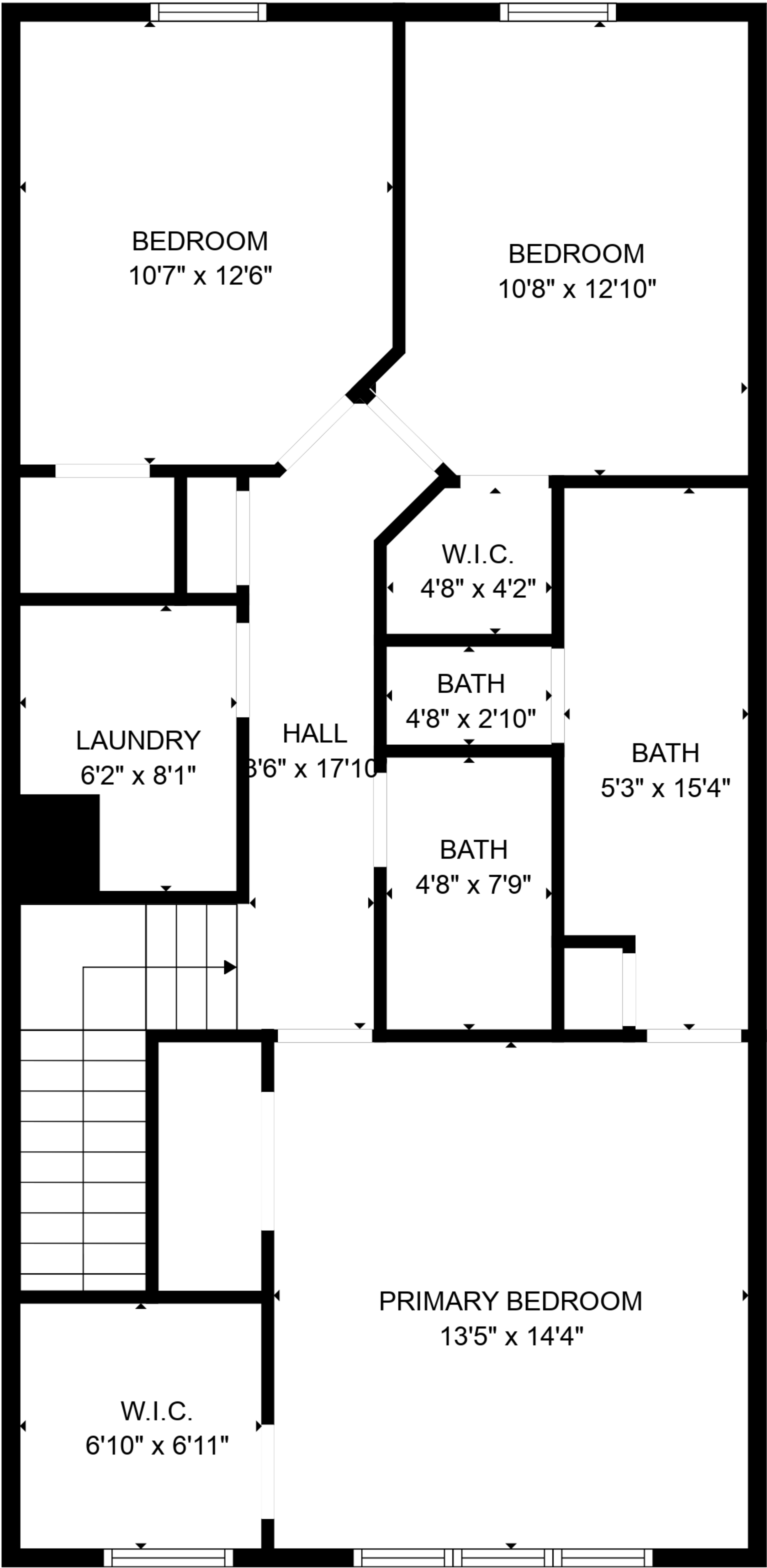
FLOOR 3
