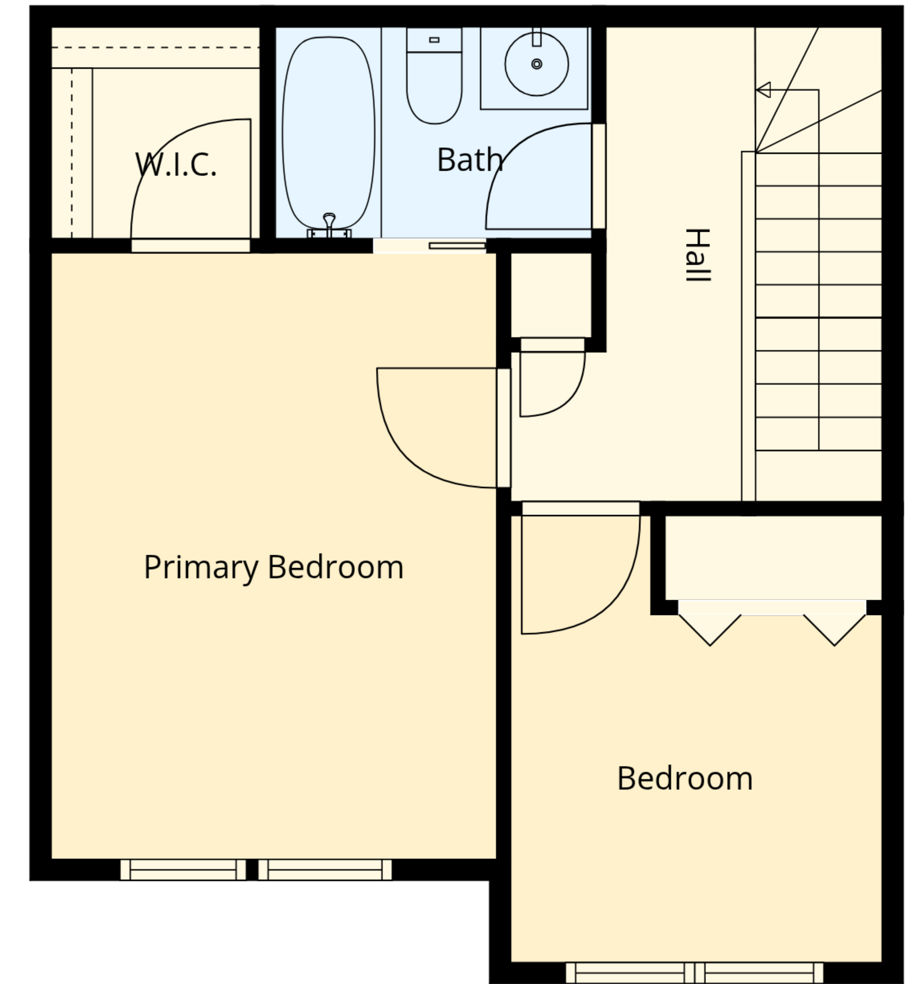
Floor 3
