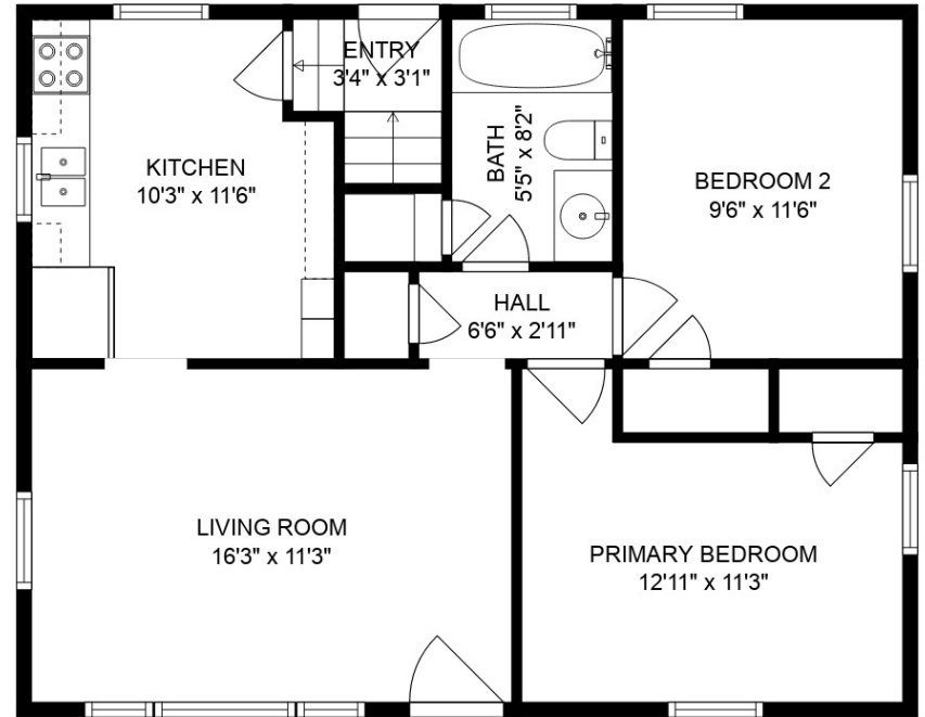
MAIN FLOOR
