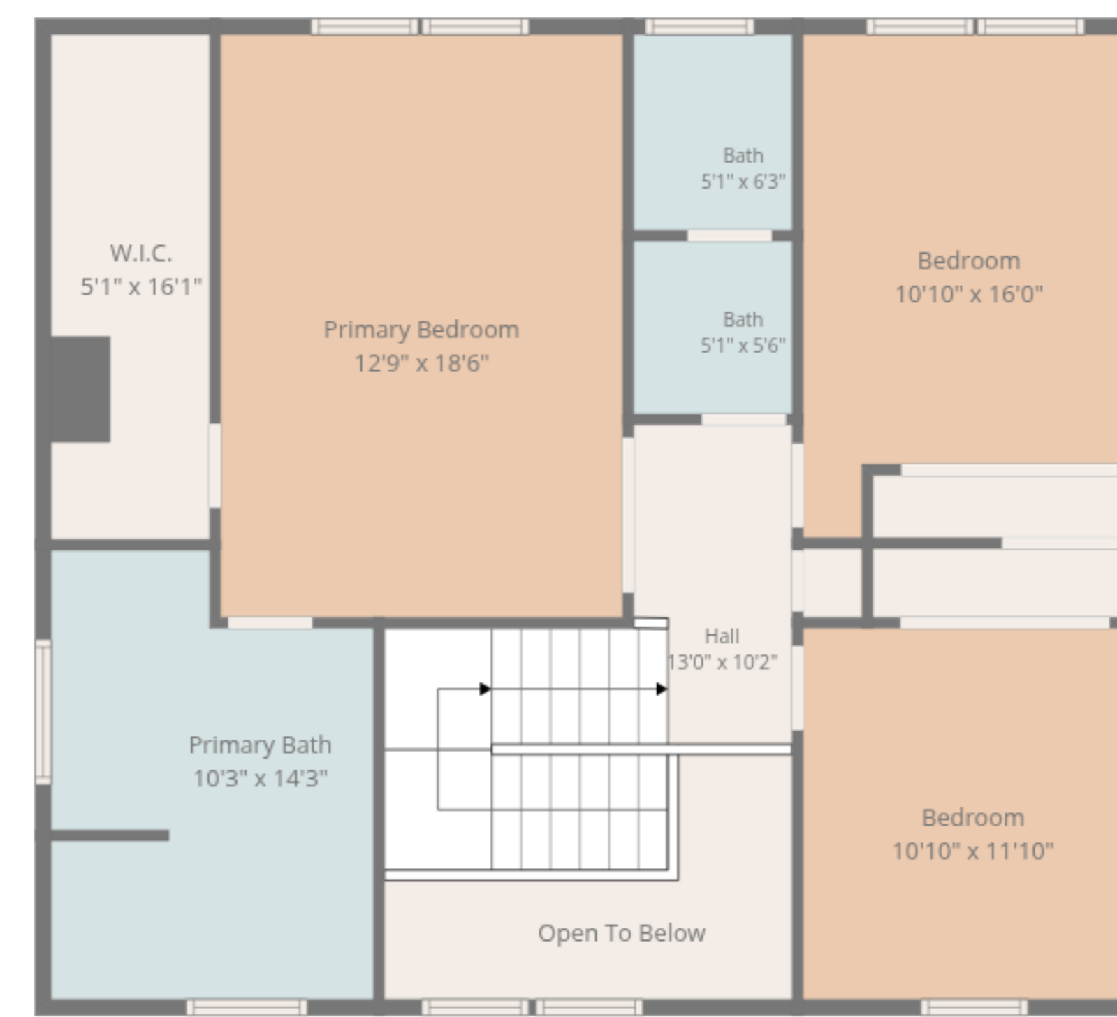
2nd Floor
