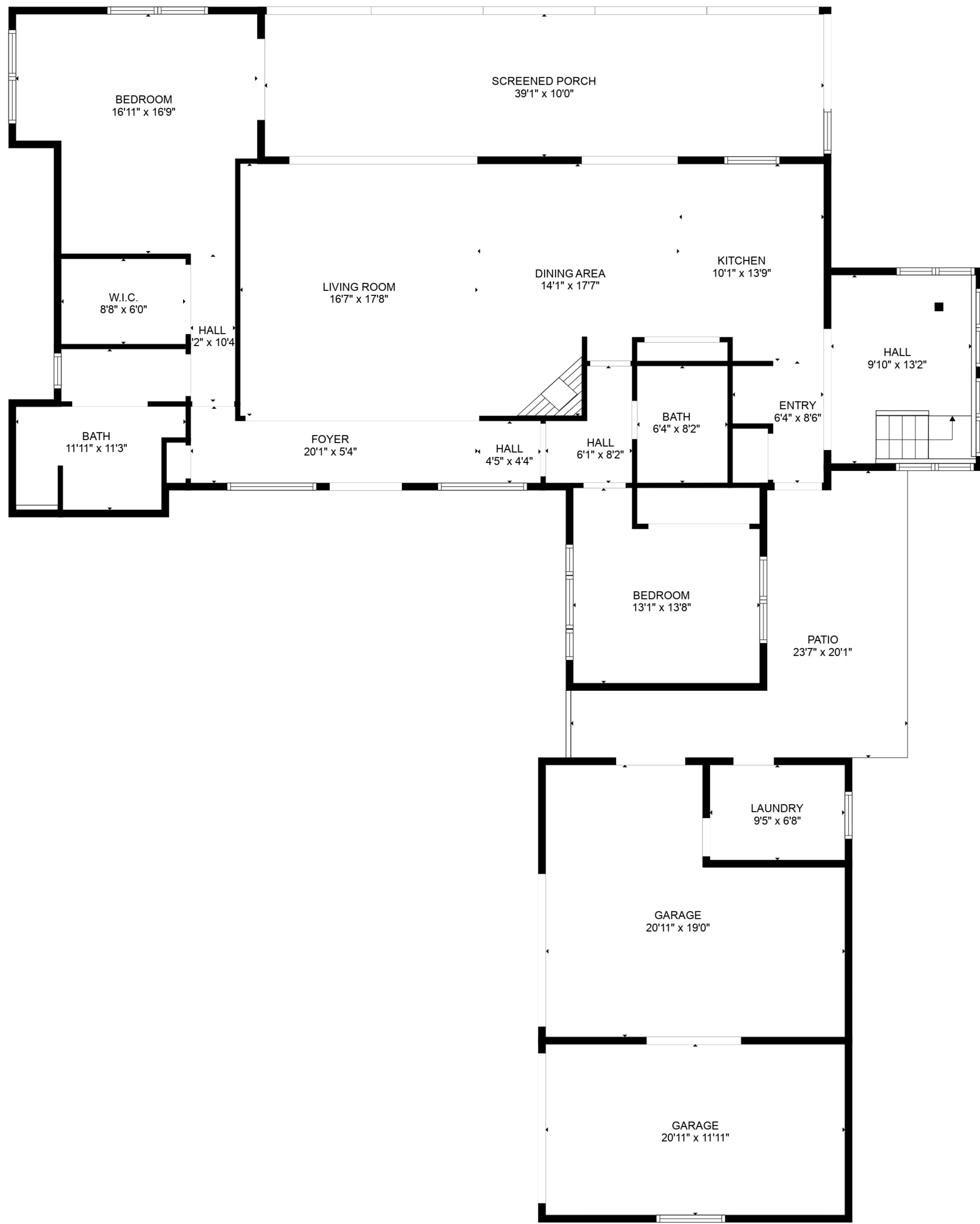
FLOOR 1
