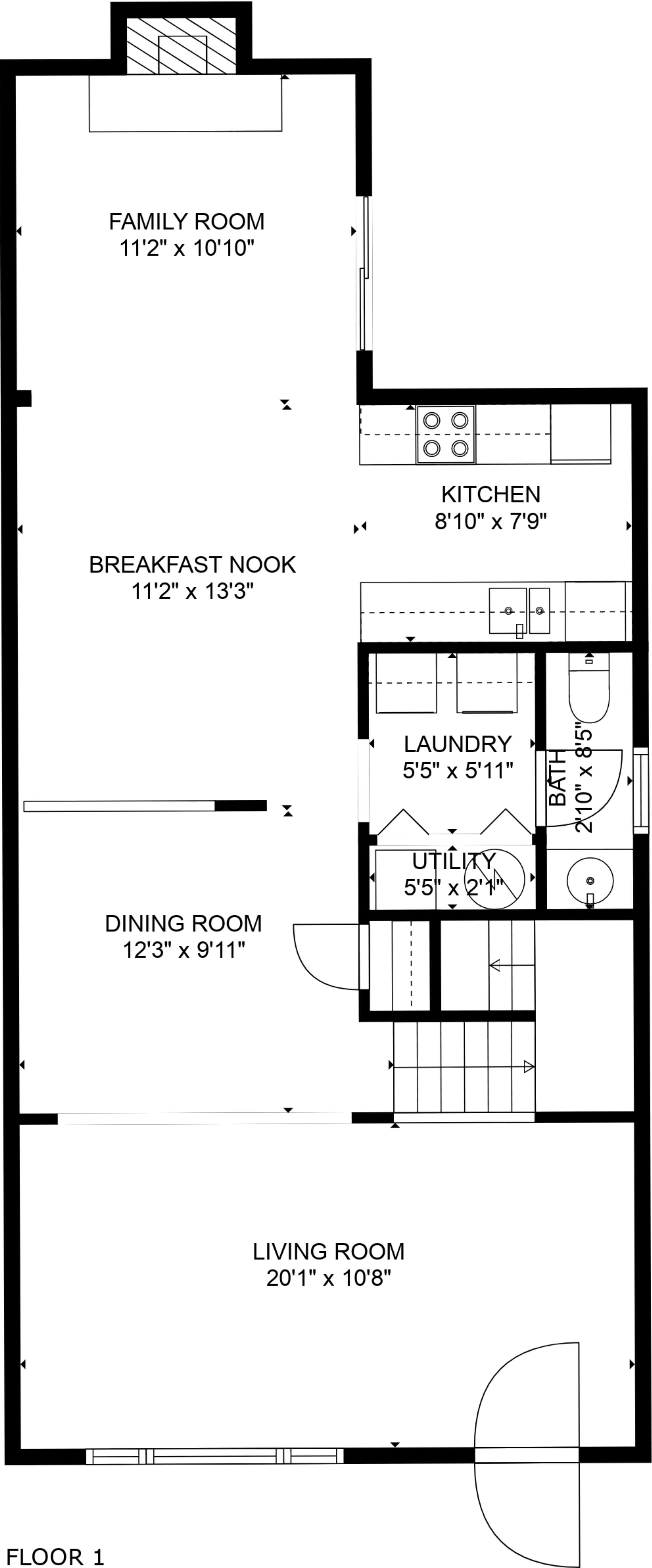
FLOOR 1
