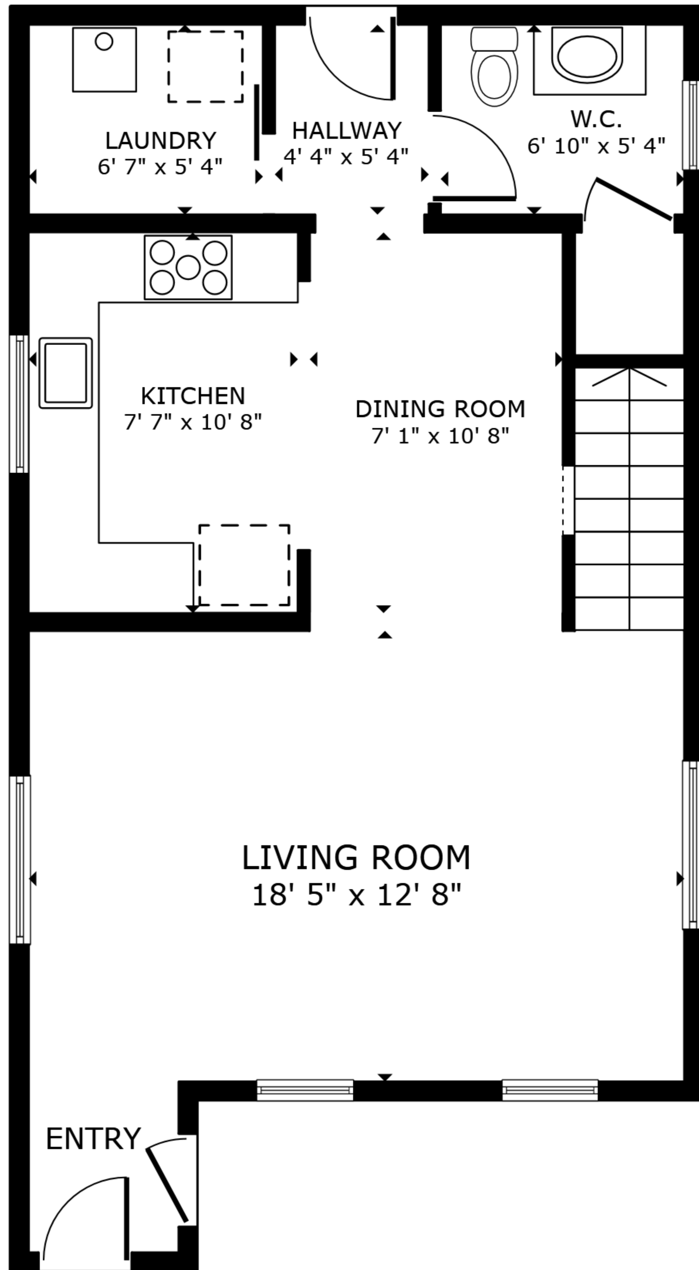
FLOOR 1
