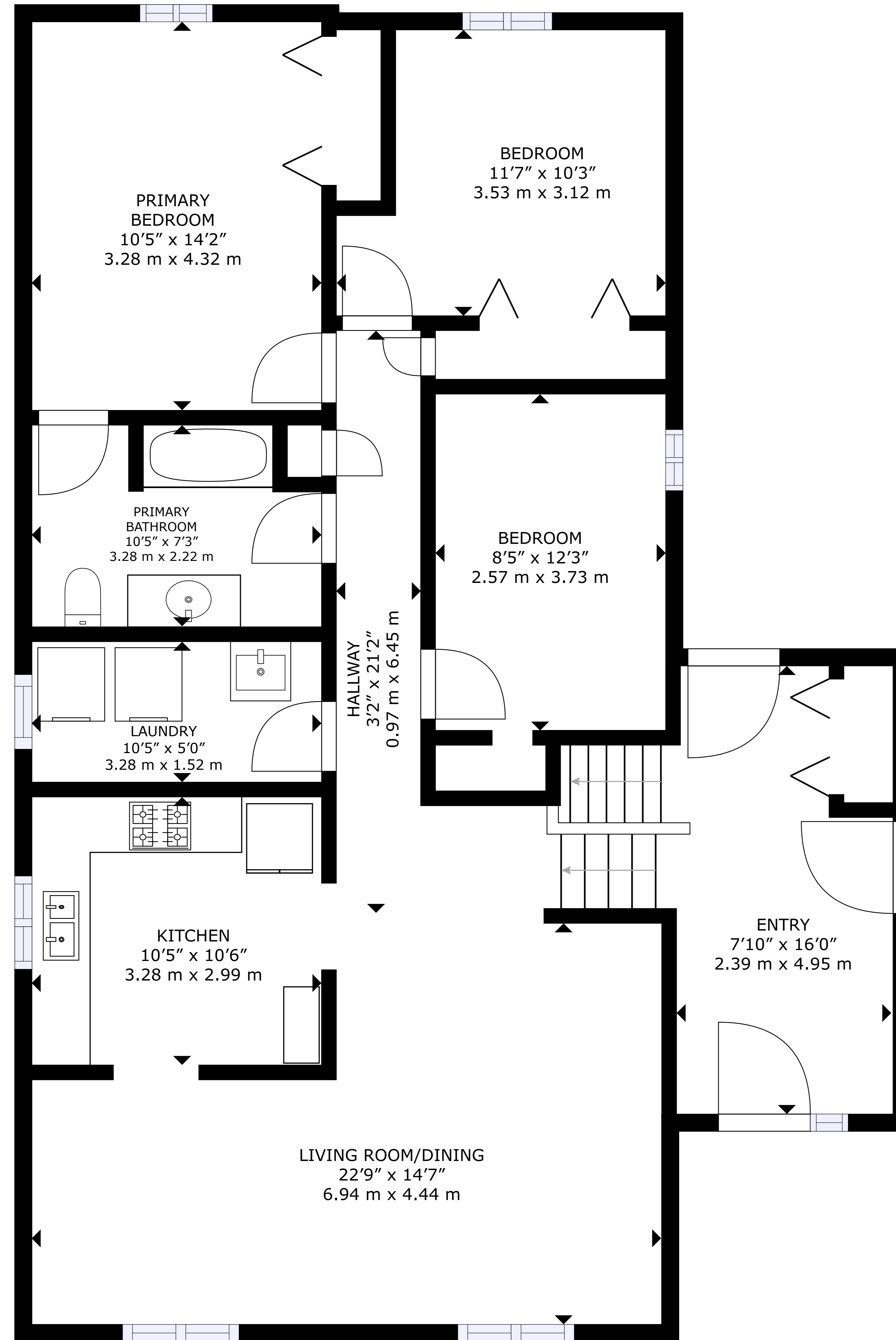
1ST FLOOR
