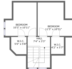
FLOOR 4
