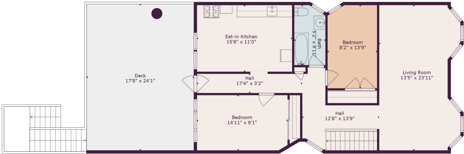
Floor 2
