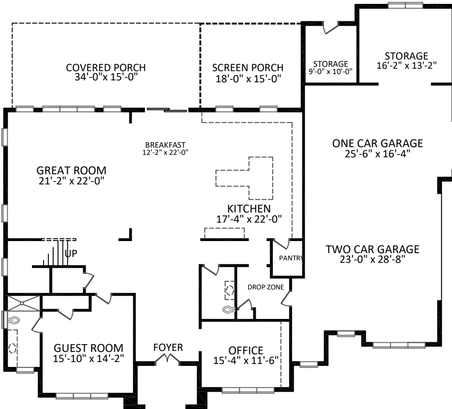
1ST FLOOR
