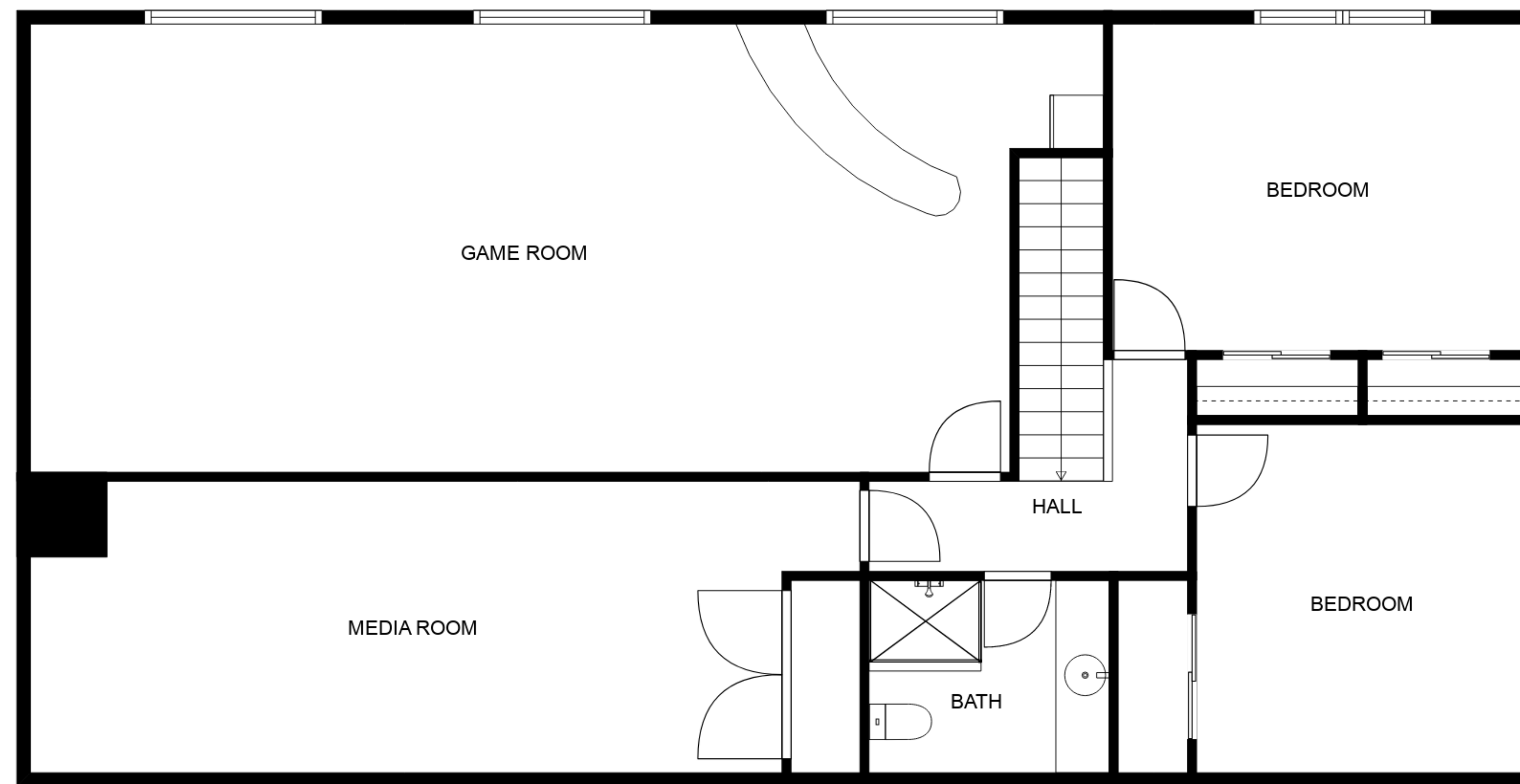
FLOOR 2
