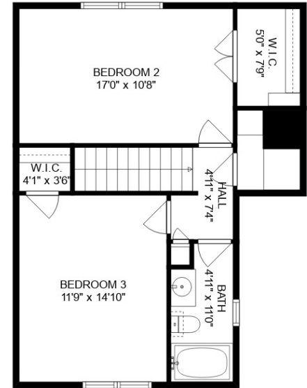
UPPER FLOOR
