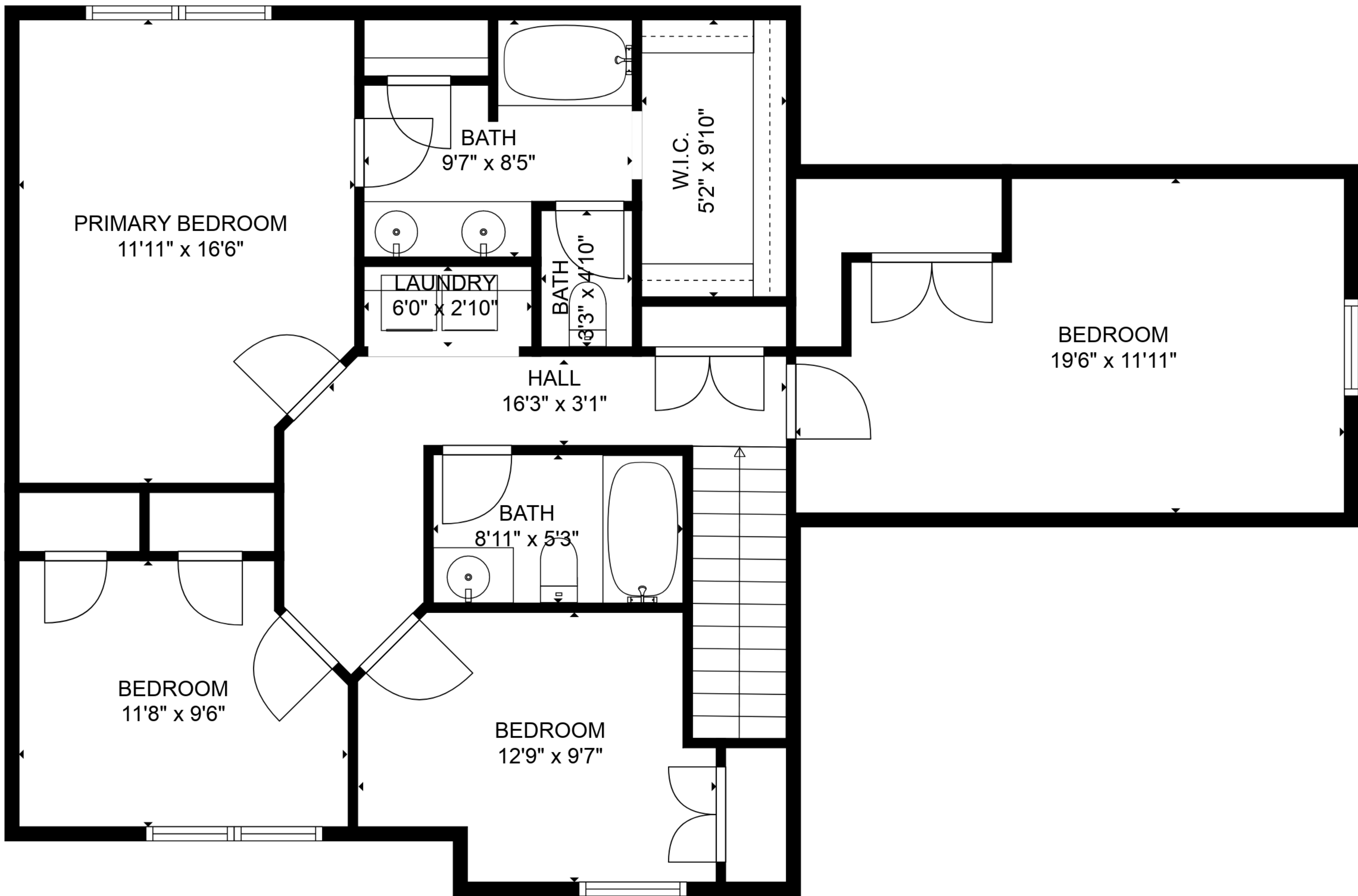
FLOOR 2
