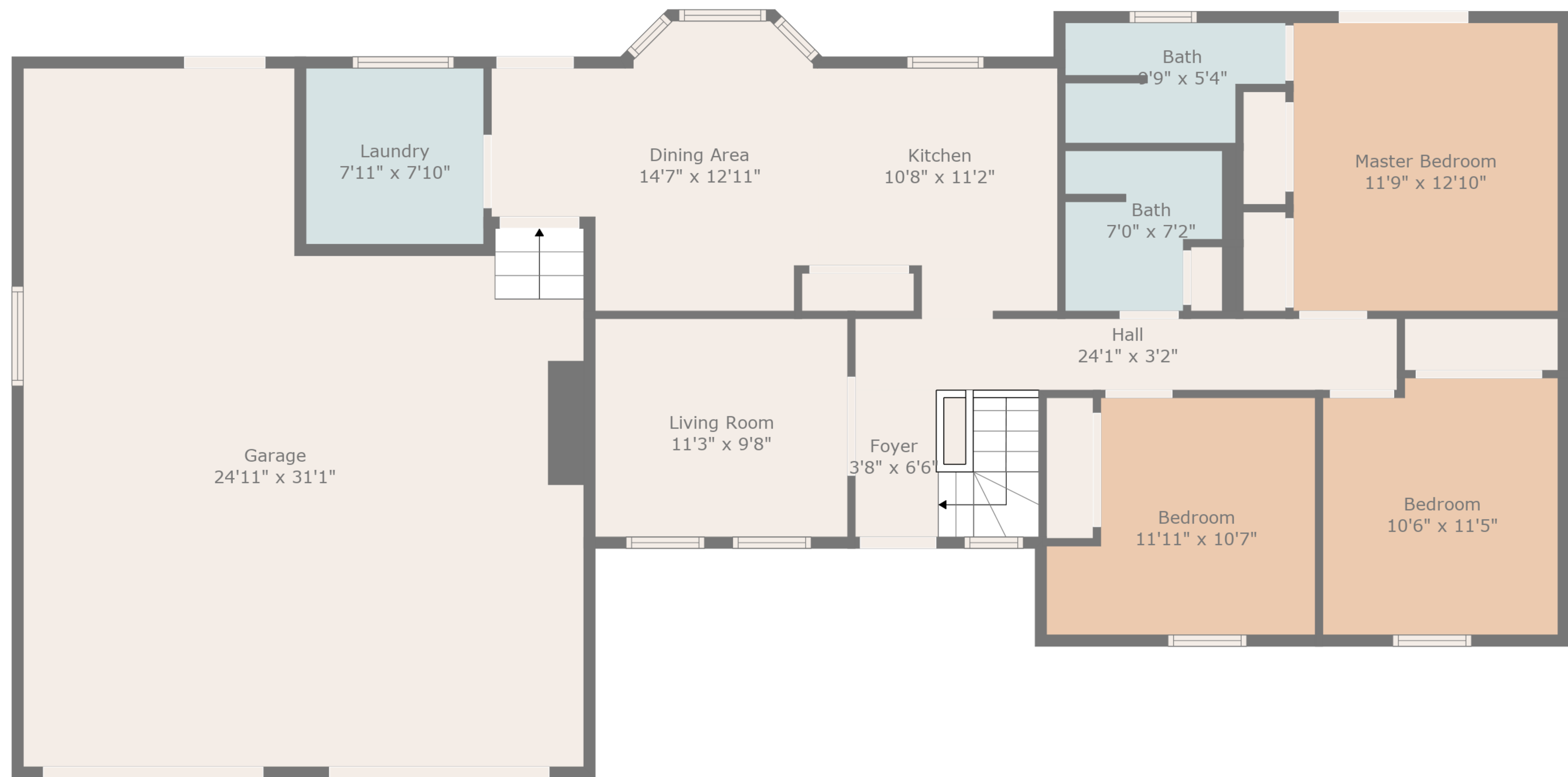
Floor 2
