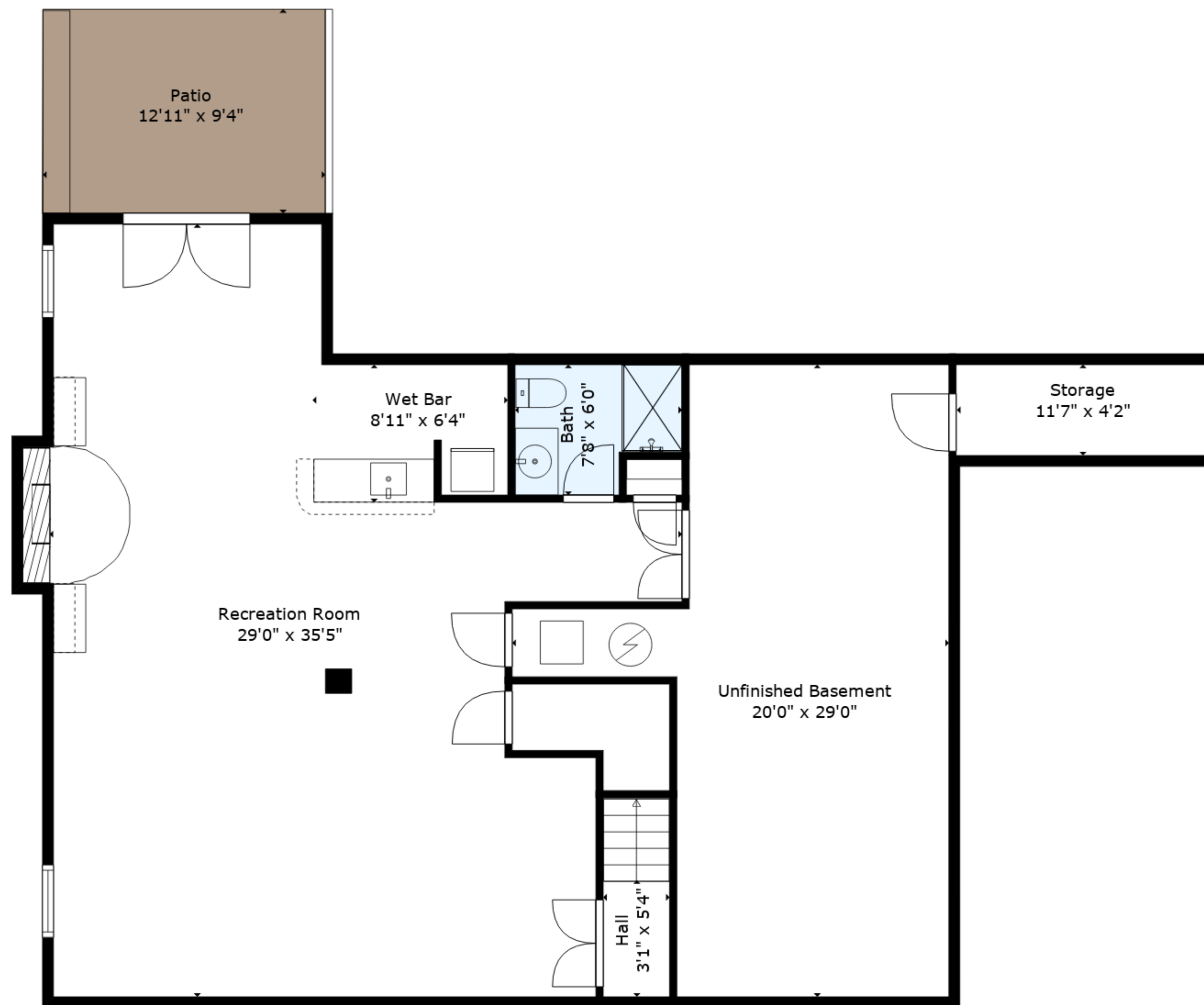
Floor 1
