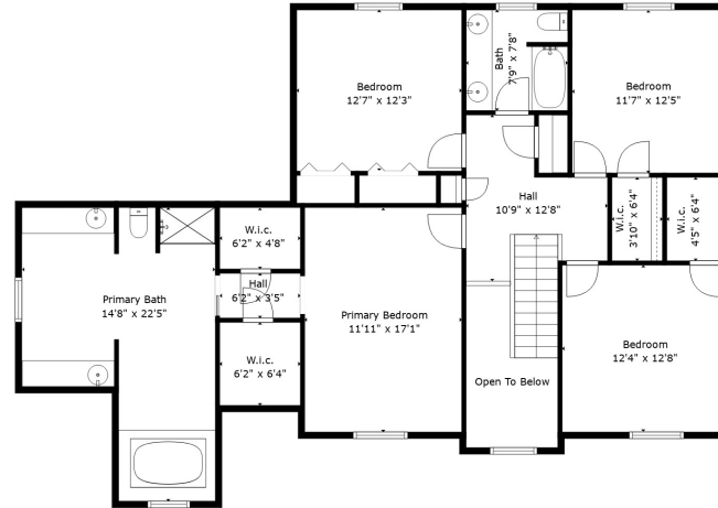
Floor 3
