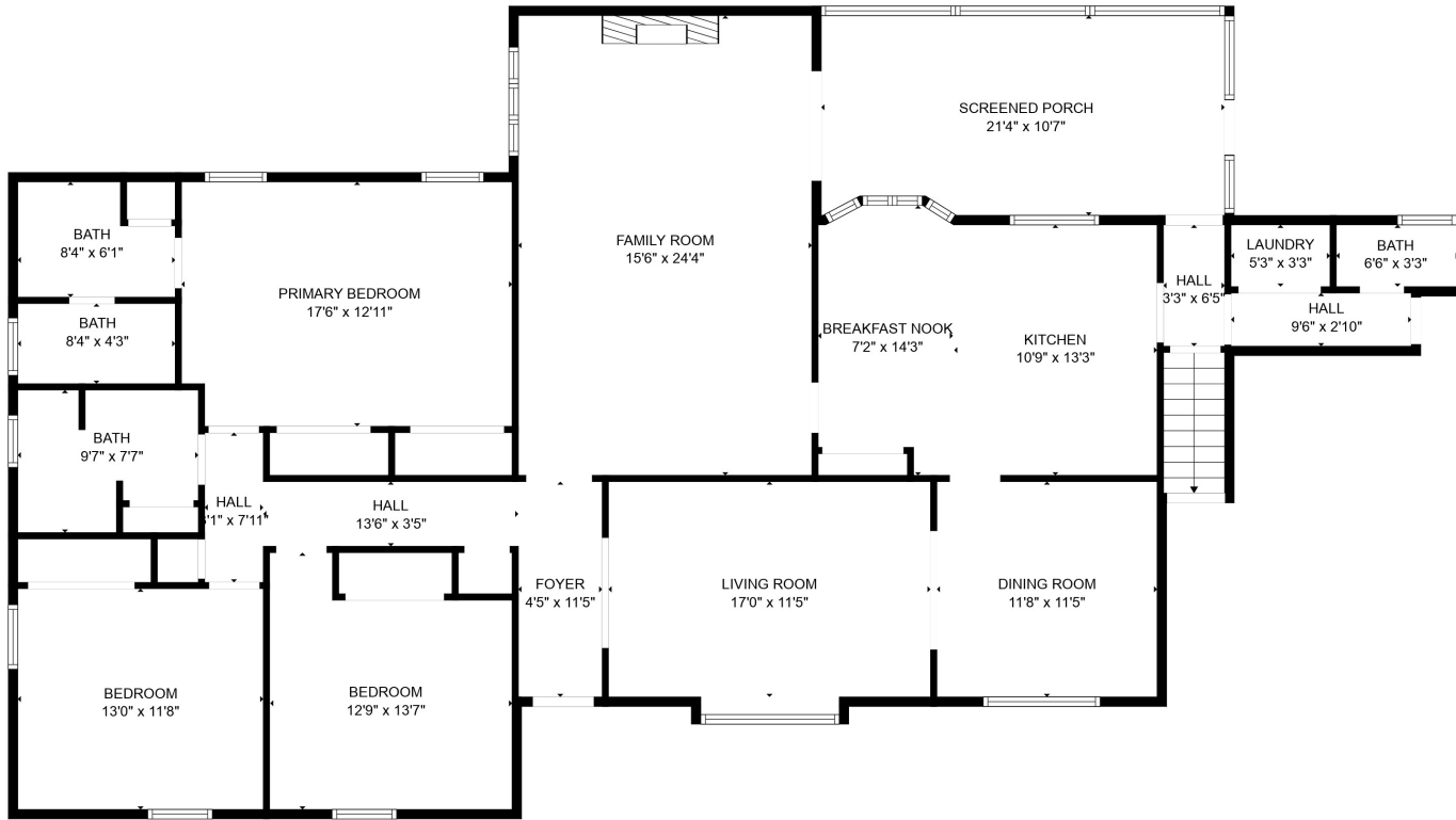
FLOOR 1
