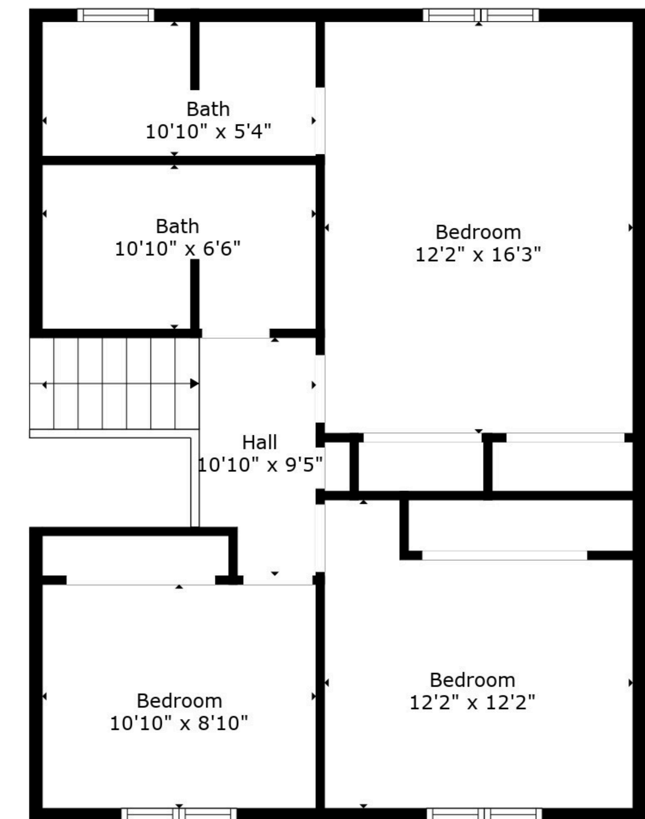
Floor 4
