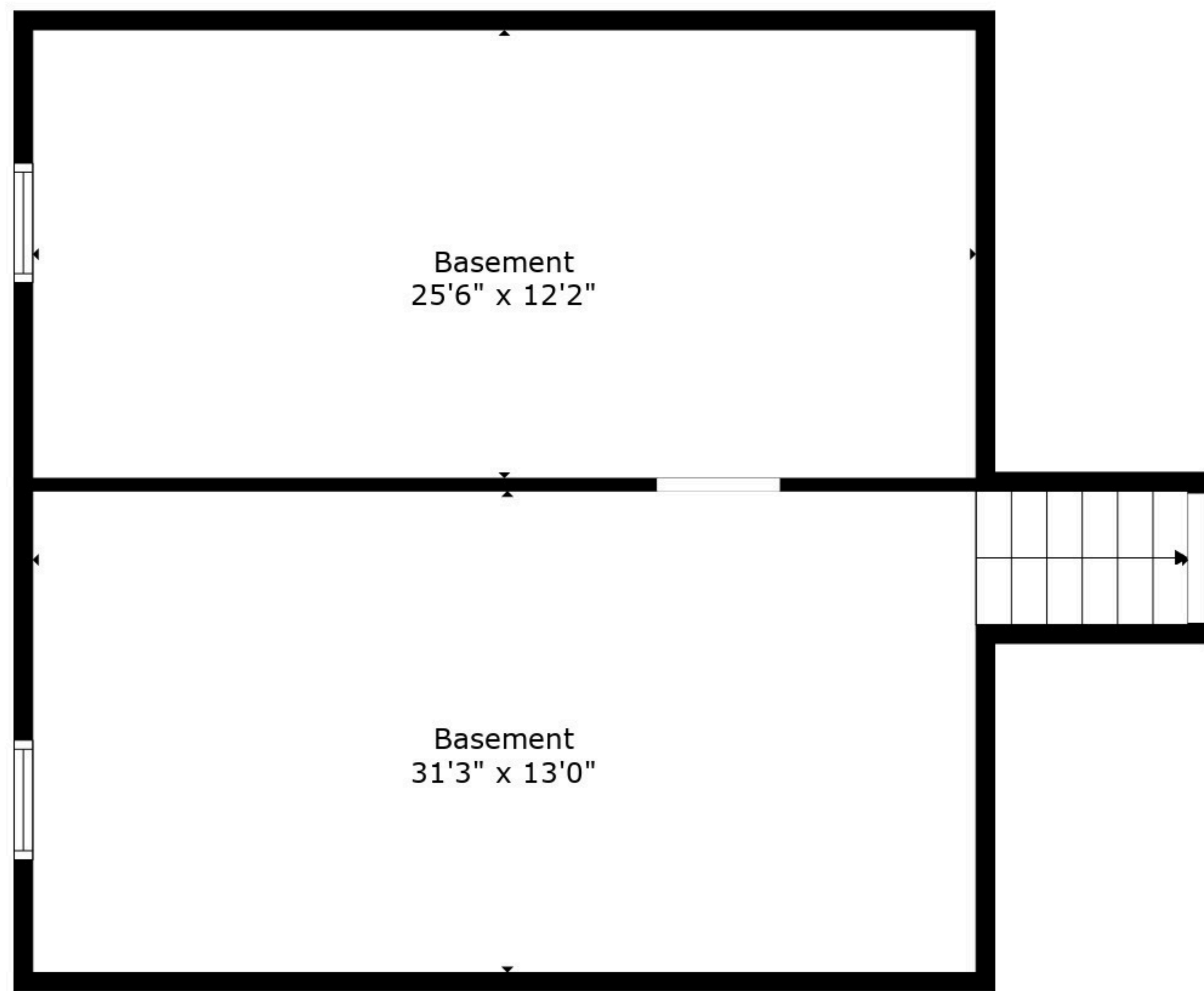
Floor 1
