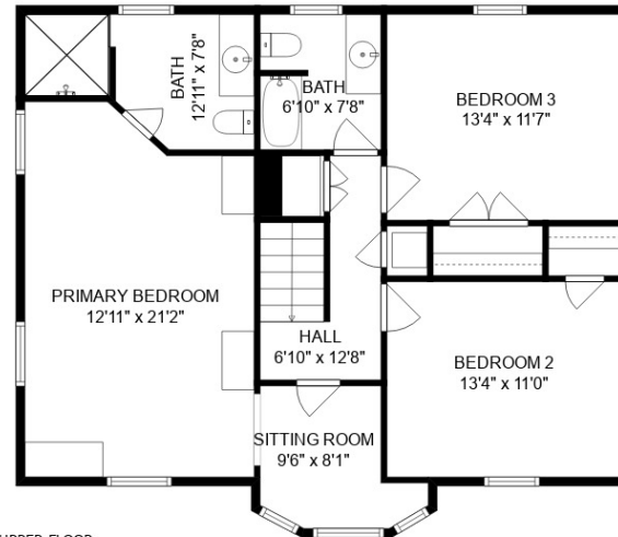
UPPER FLOOR
