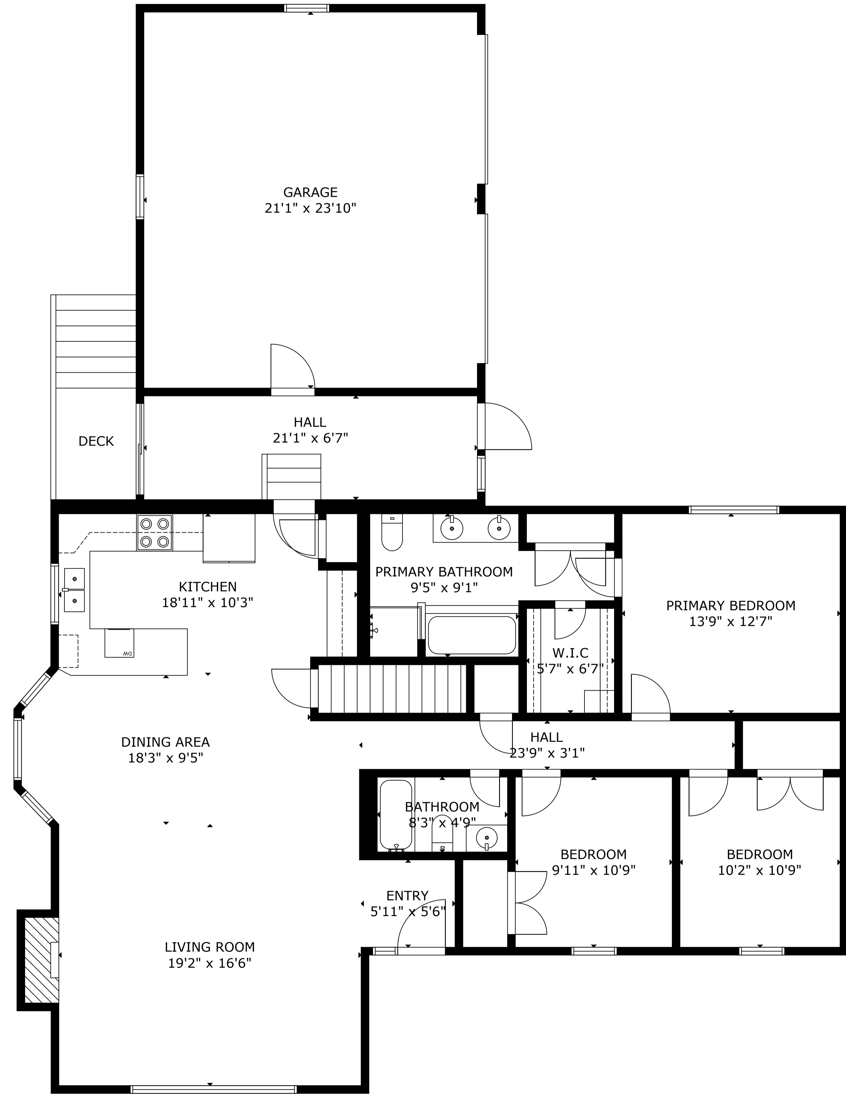
MAIN FLOOR
