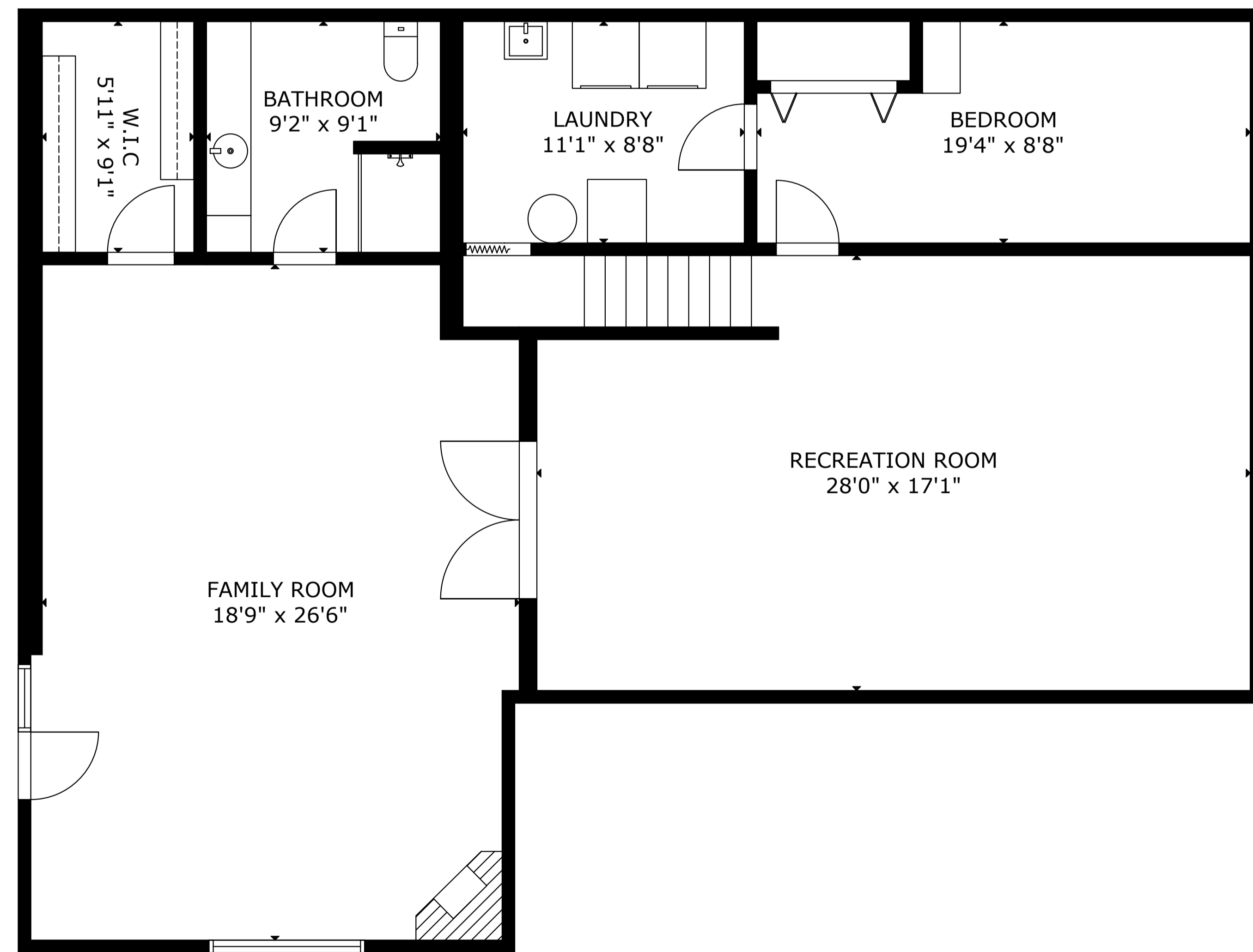
LOWER FLOOR
