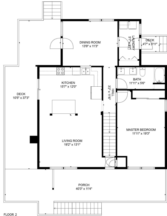
FLOOR 2
