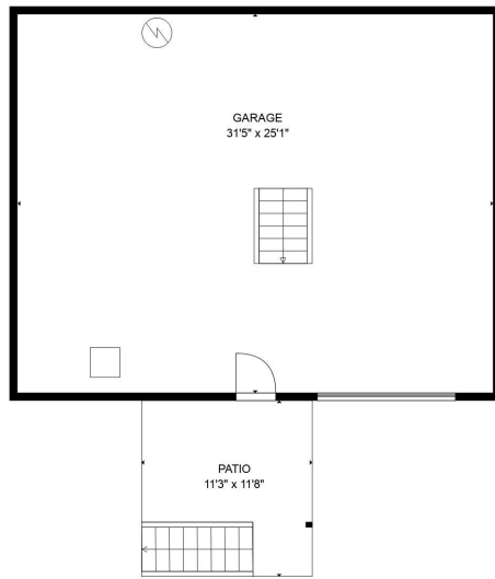
FLOOR 1
