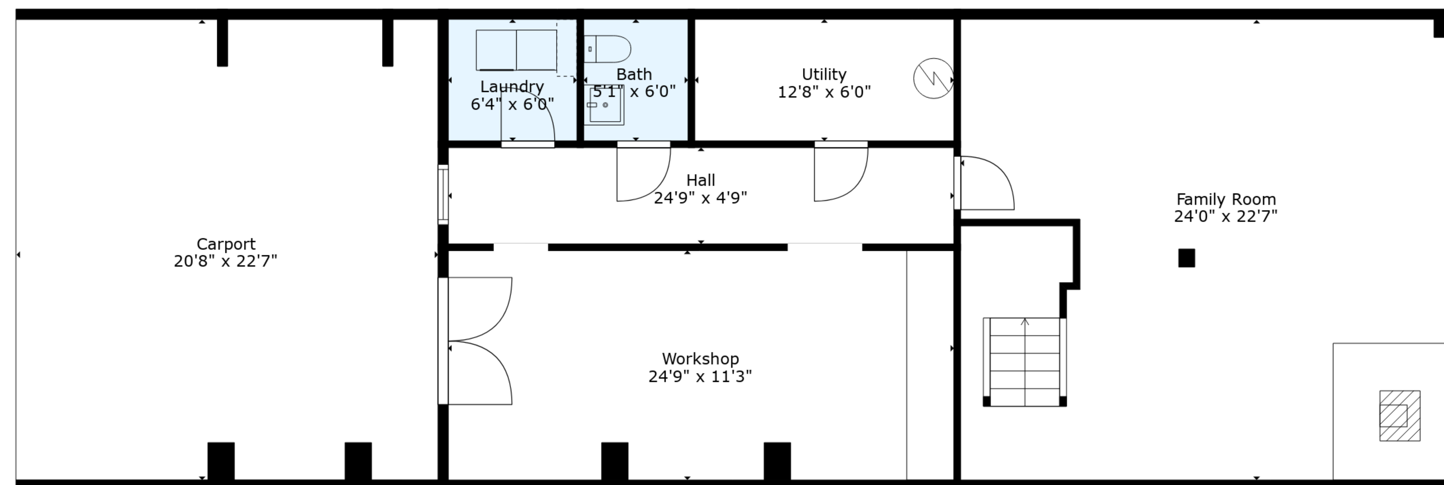
Floor 1
