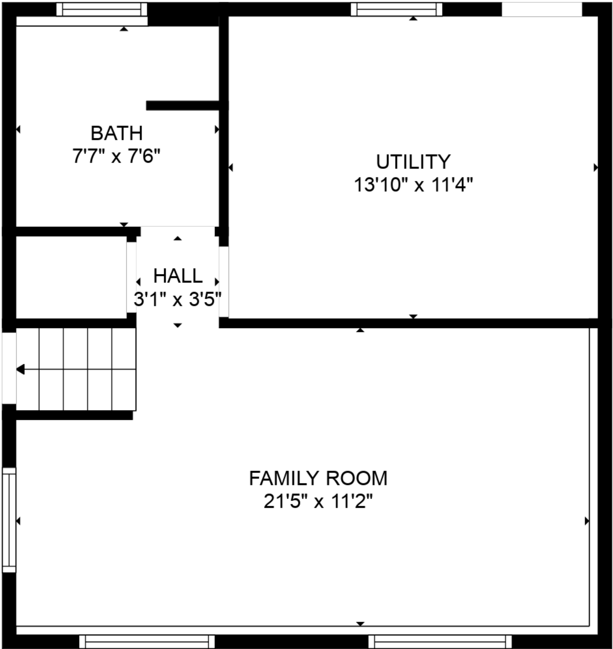
FLOOR 3
