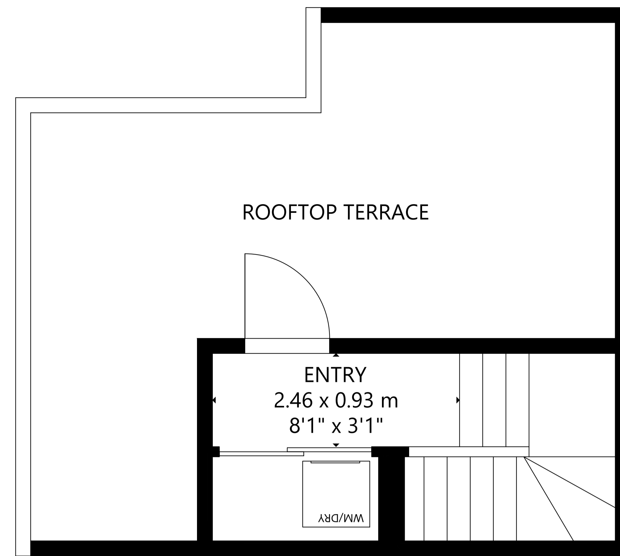
THIRD FLOOR
