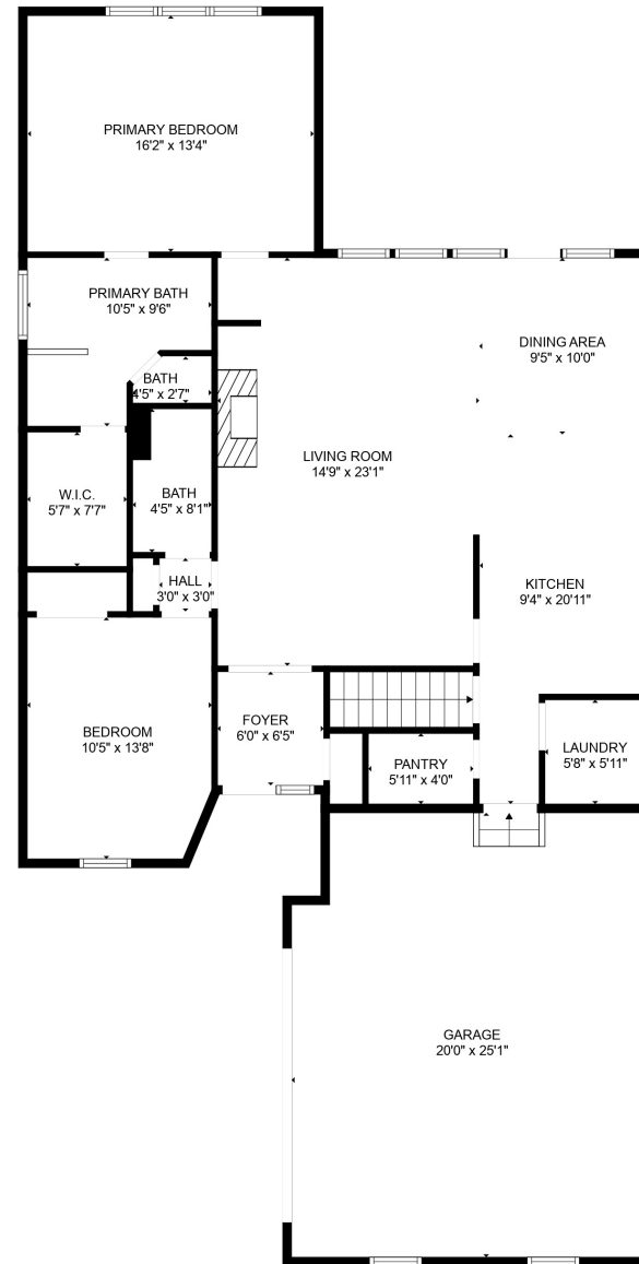
FLOOR 2
