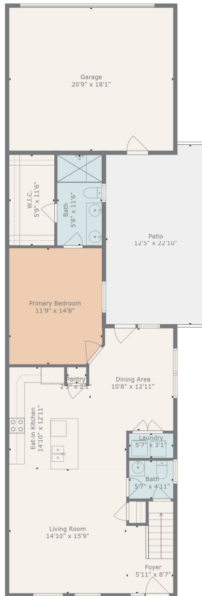
Floor 1
