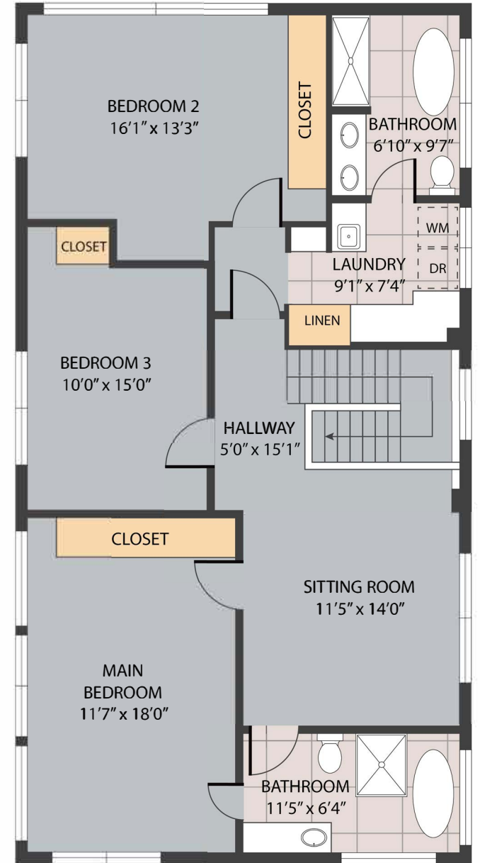
SECOND FLOOR
